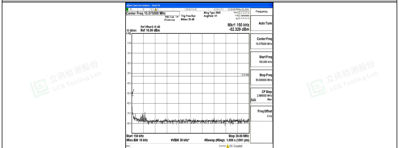
Band2_1.4MHz_QPSK_19193_1RB#0_0.15~30_0.15~30
