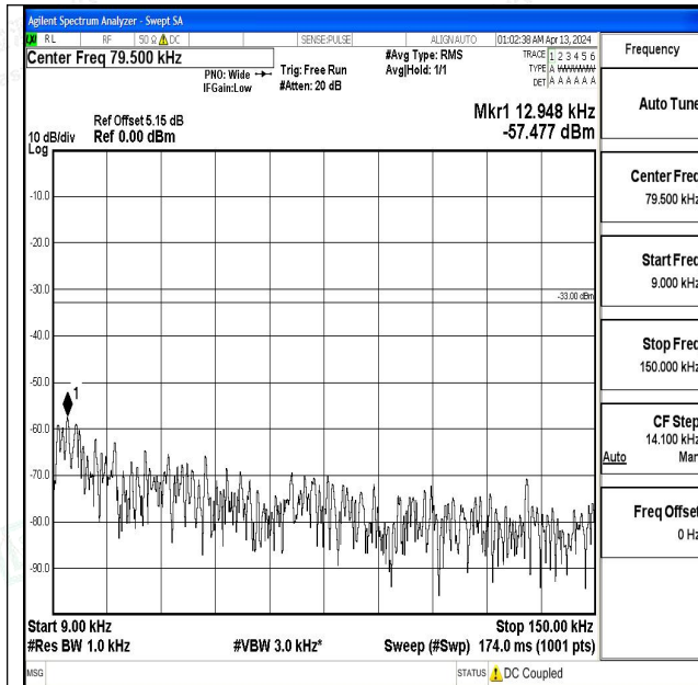
Band71_10MHz_QPSK_133172_1RB#0_0.009~0.15_0.0 09~0.15
