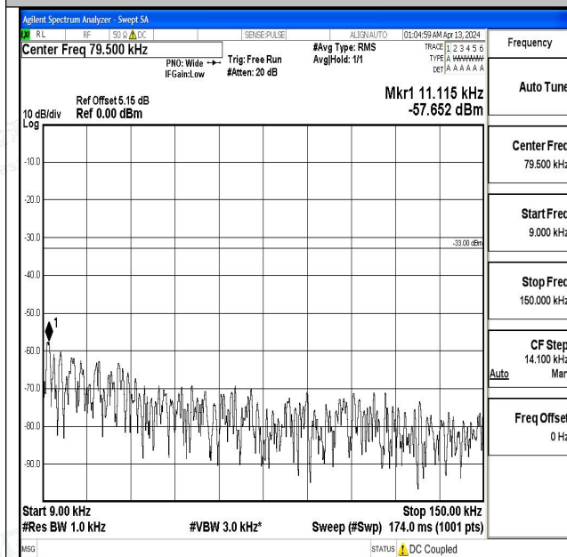
Band71_10MHz_QPSK_133297_1RB#0_0.009~0.15_0.0 09~0.15
