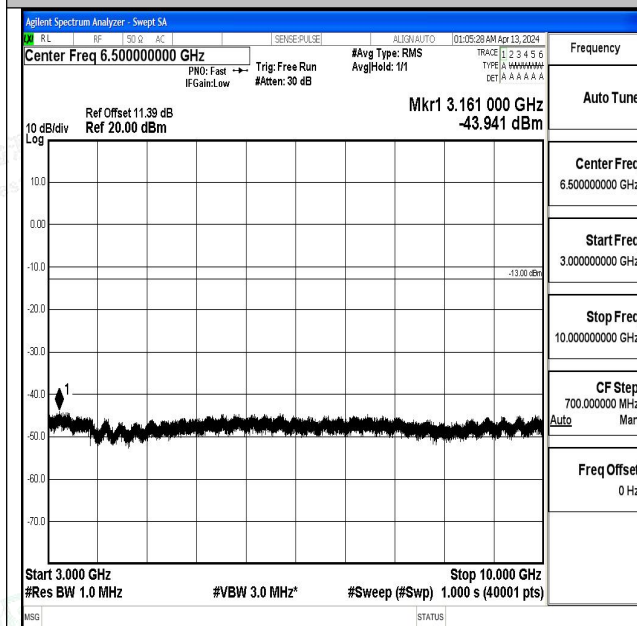
Band71_10MHz_QPSK_133297_1RB#0_3000~10000_3000~10000
