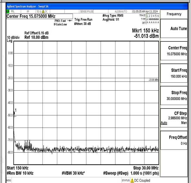
Band71_10MHz_QPSK_133297_1RB#0_0.15~30_0.15~ 30
