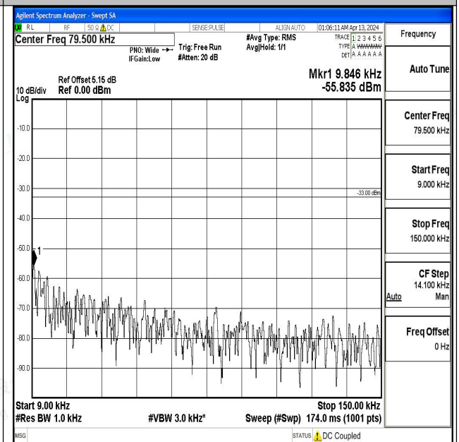
Band71_10MHz_16QAM_133297_1RB#0_0.009~0.15_0.009~0.15
