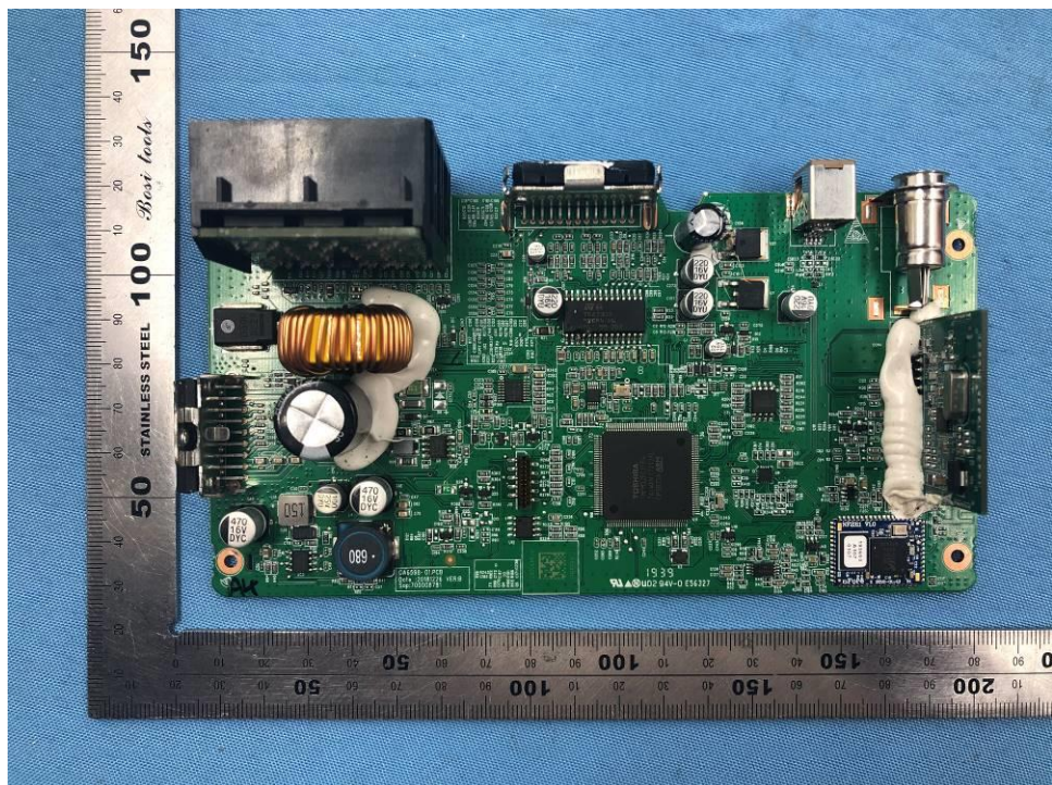
PCB view-1
