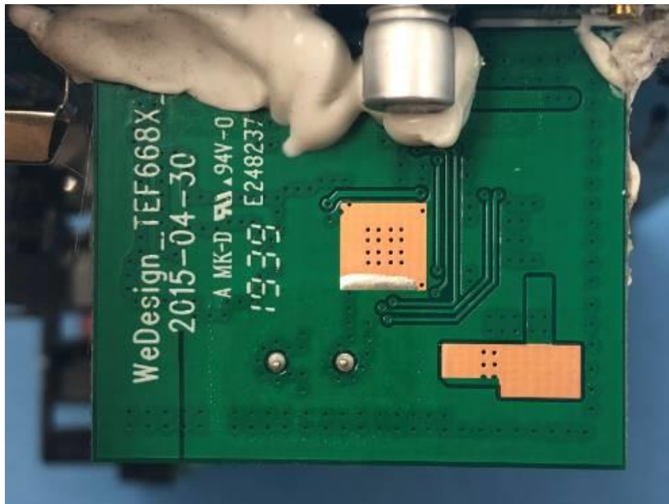
PCB view-4
