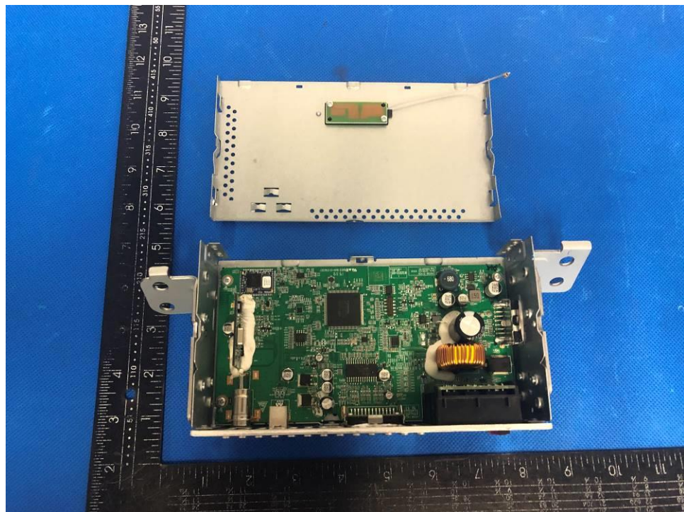
Internal view-2
