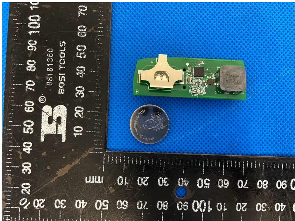
PCB and battery view
