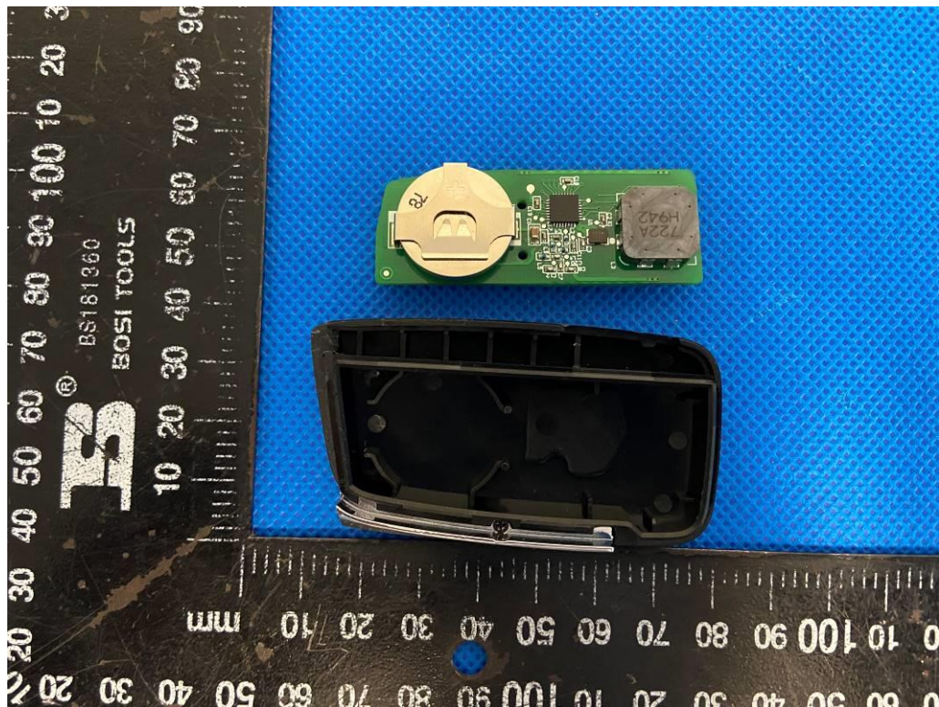
Internal view-3
