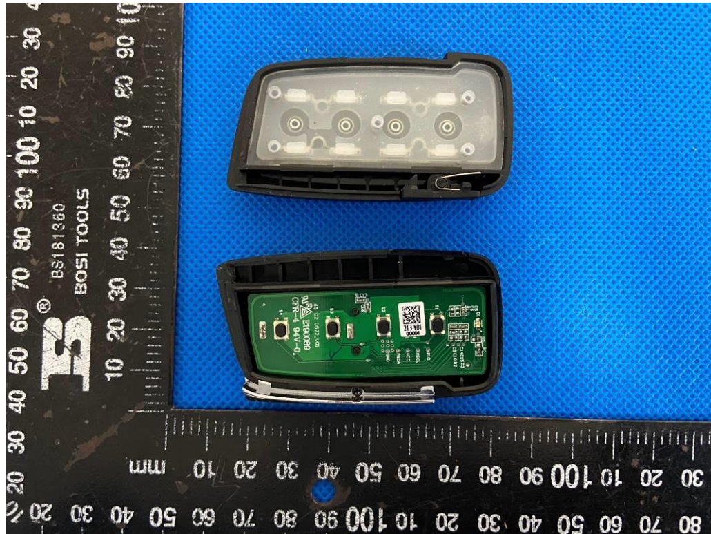
Internal view -1
