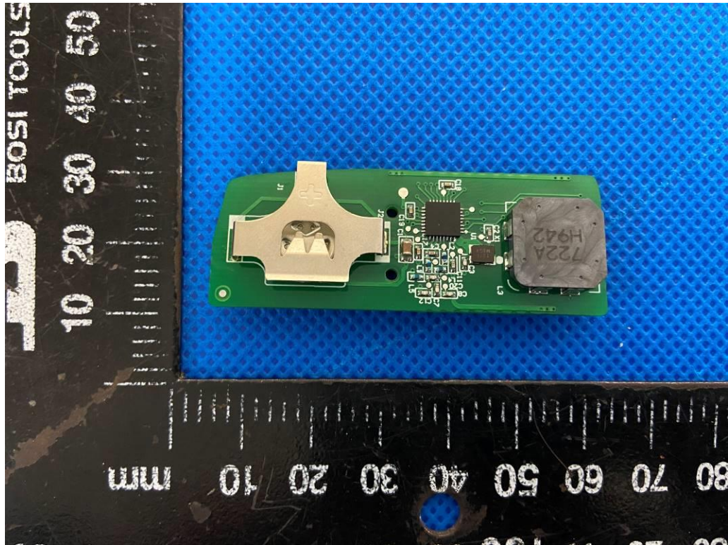
PCB view-1
