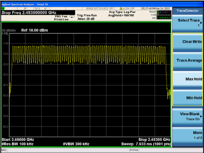
GFSK Modulation
