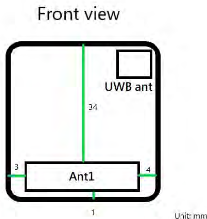
Fig.12 Antenna position of EUT
