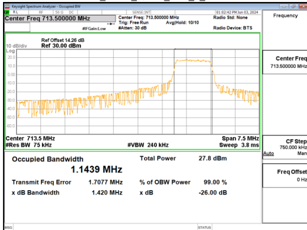
Band12_5MHz_QPSK_RB6_0_CH23155
