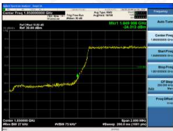
LCH_QPSK_6RB#0
