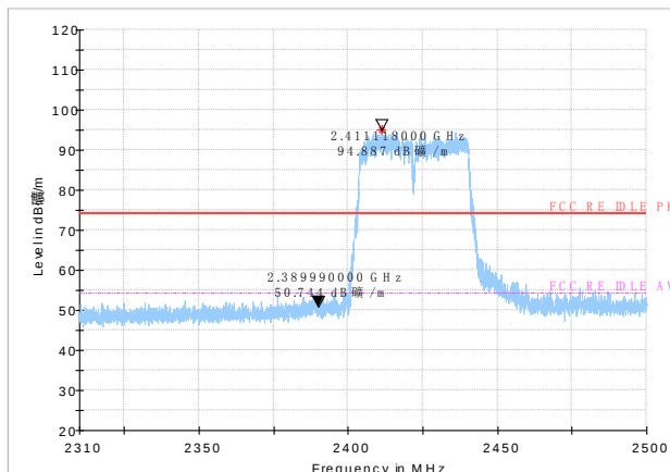
Peak detector
