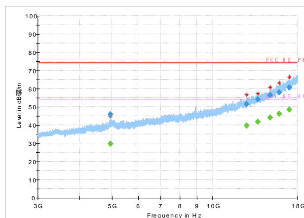
Radiated emission (High): \pi/4 DQPSK, high channel
