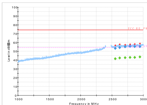
Radiated emission (Low): 8DPSK, low channel
