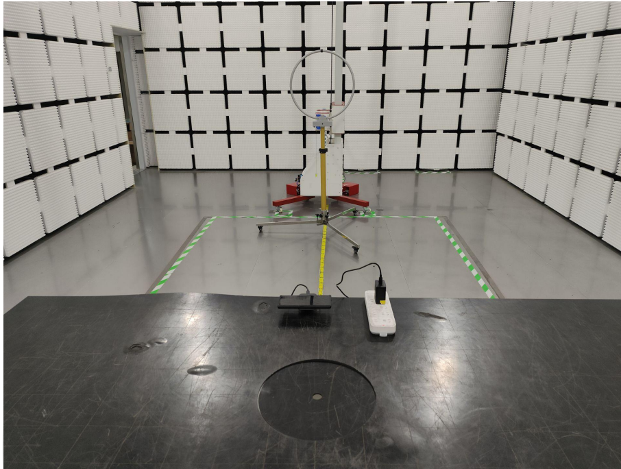
Spurious Radiation Emissions Test (9KHz-30MHz)
