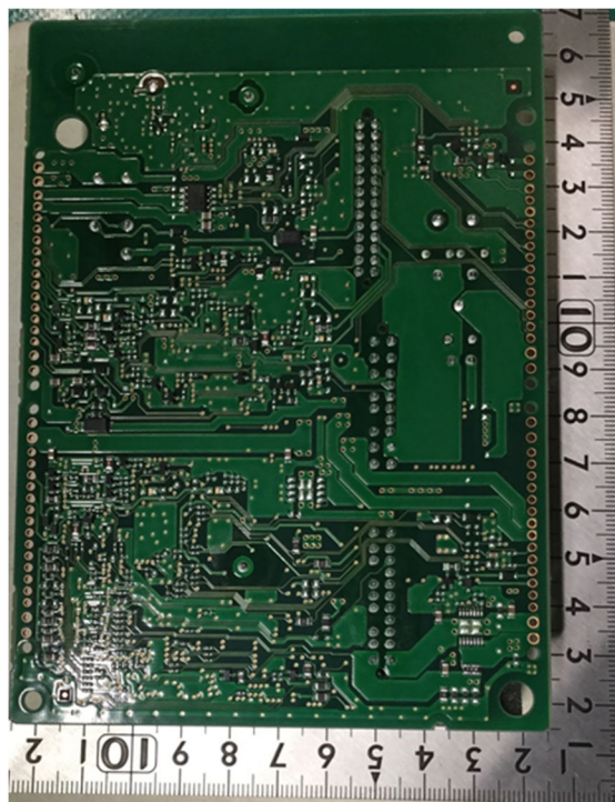
Solder side
