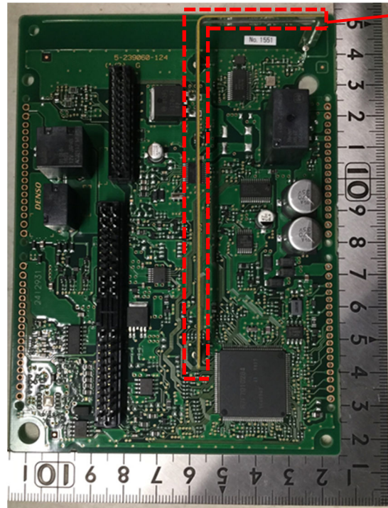
Component side
