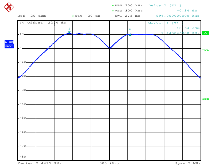
Channel Separation Plot on Channel 39 - 40
