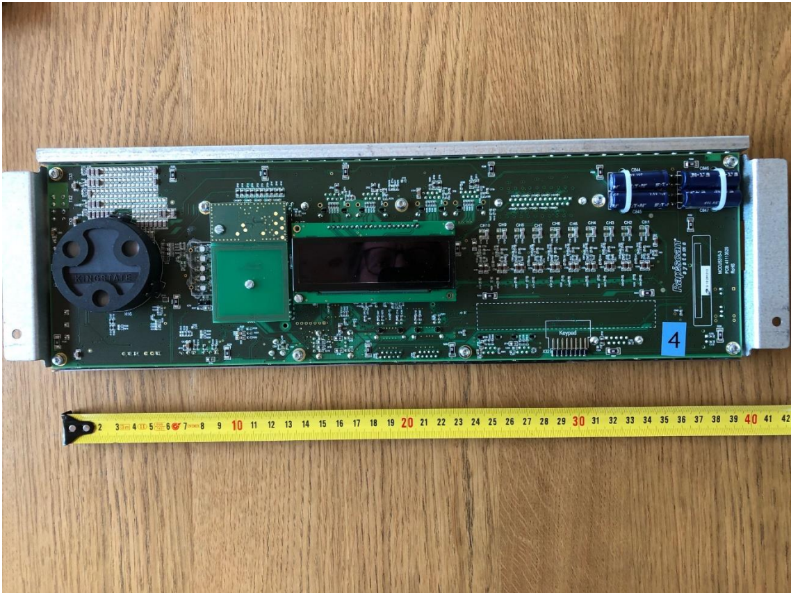
Main electronics component side with NFC module
