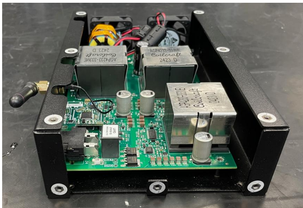
Enclosure Right Side View
