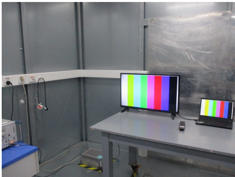
Photograph 3: Set-up photo for AC Conducted Emissions
