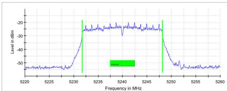
6 dB Bandwidth
