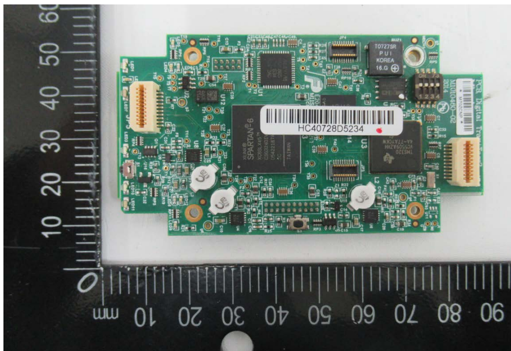
Test sample – External (Bottom)
