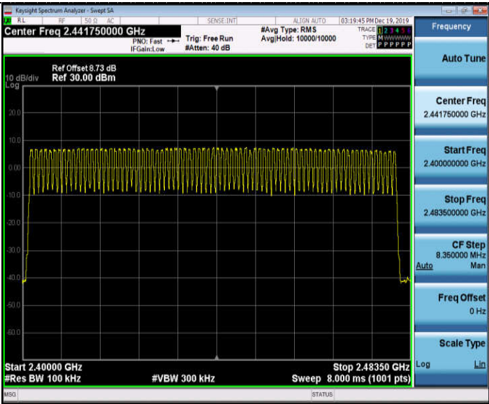
GFSK Modulation
