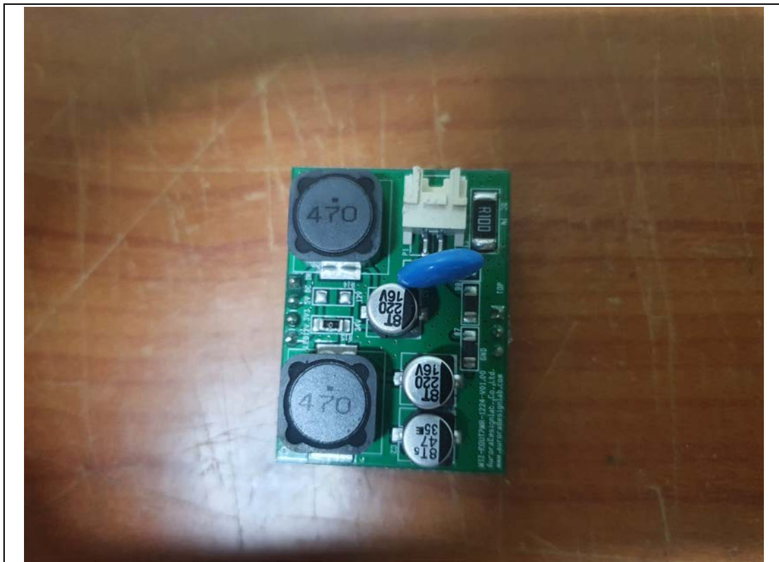
SubBoard-Rear
