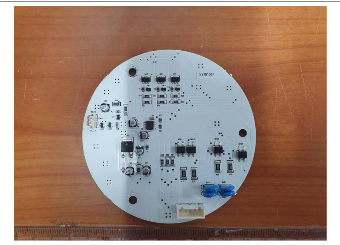
MainBoard-Rear
