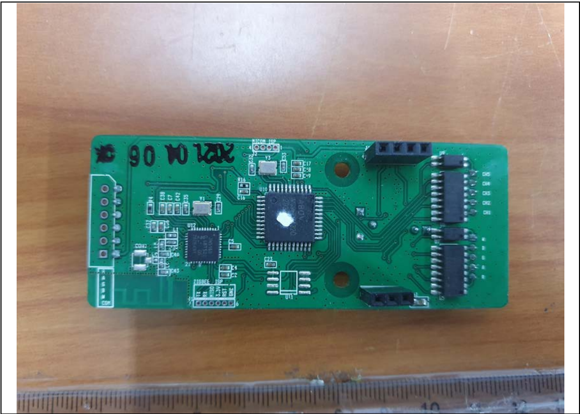
Main Board–Rear
