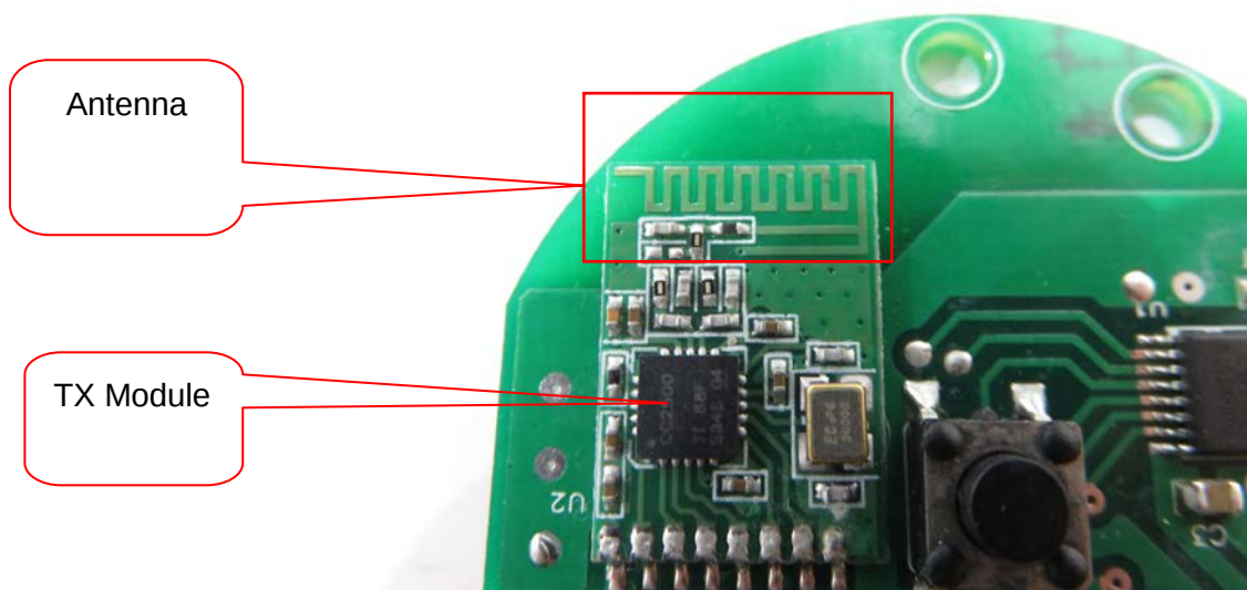
Close Up View of the TX module & Antenna
