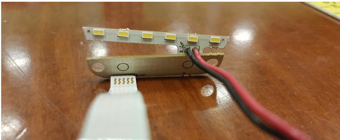
Figure 5 – EUT Internal Photo Bottom Touch Sensor and LED Boards
