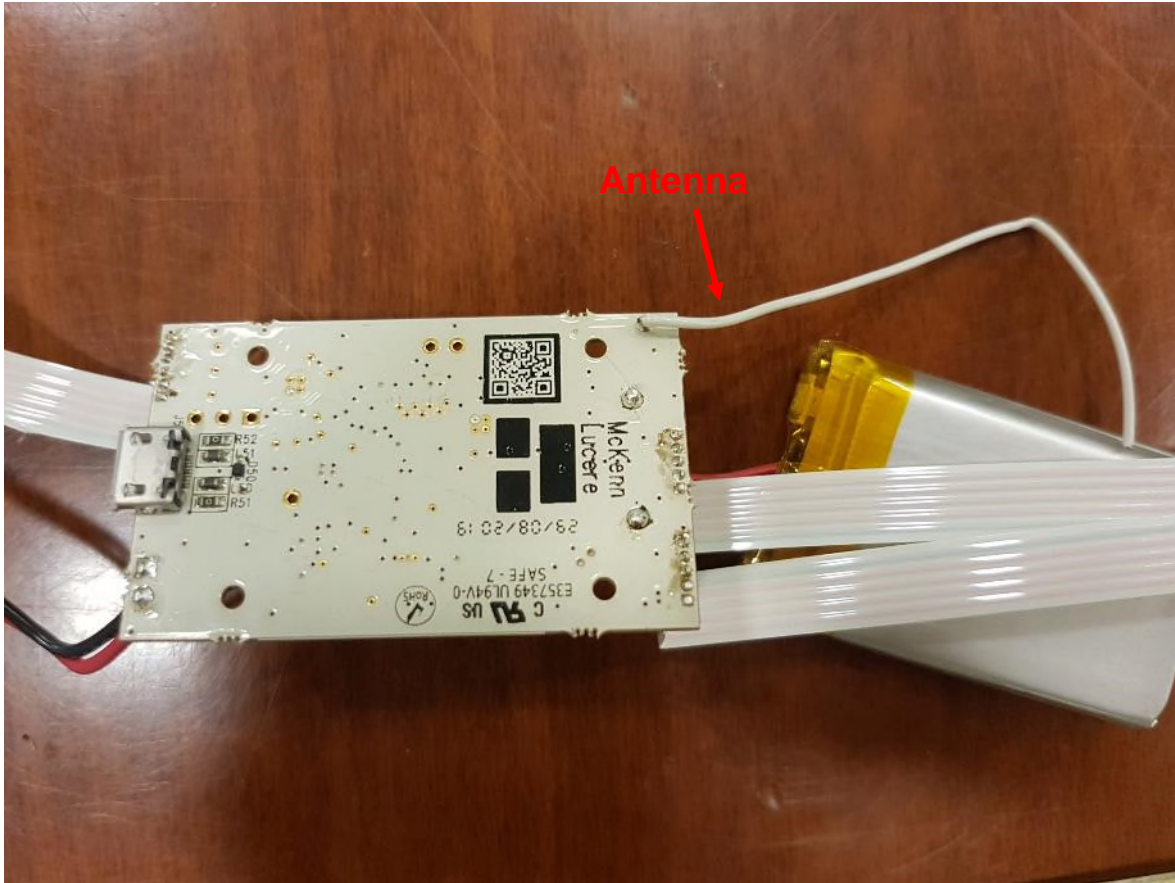
Figure 3 – EUT Internal Photo Back
