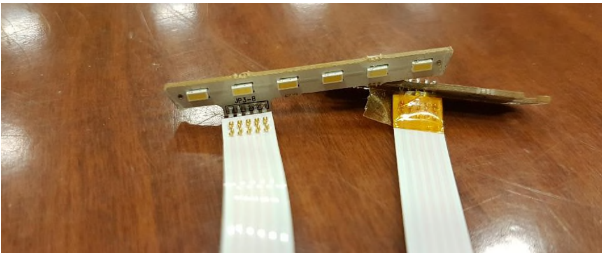
Figure 4 – EUT Internal Photo Top Touch Sensor and LED Boards
