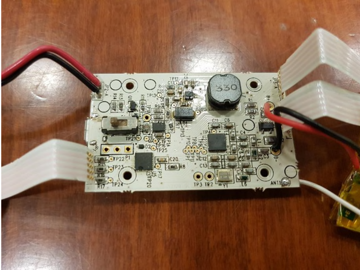
Figure 1 – EUT Internal Photo Main Board - Front
