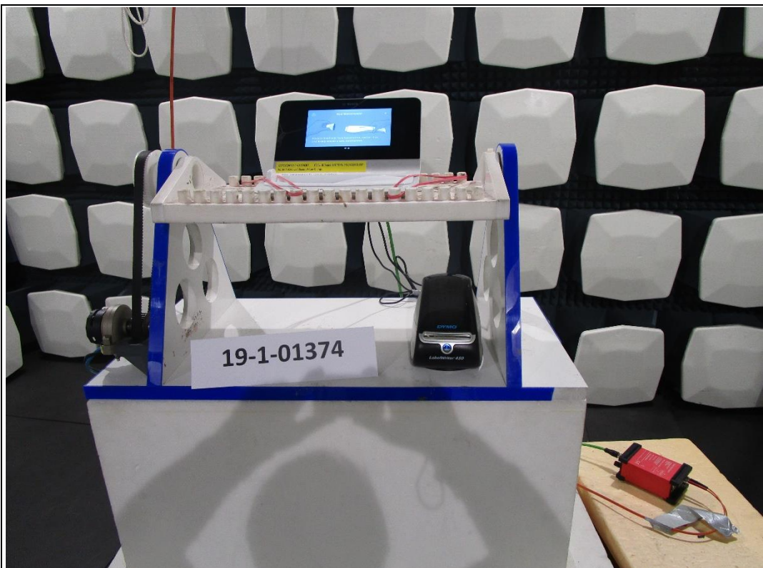
Photograph 4: Radiated measurements test set-up above 1 GHz, close up view
