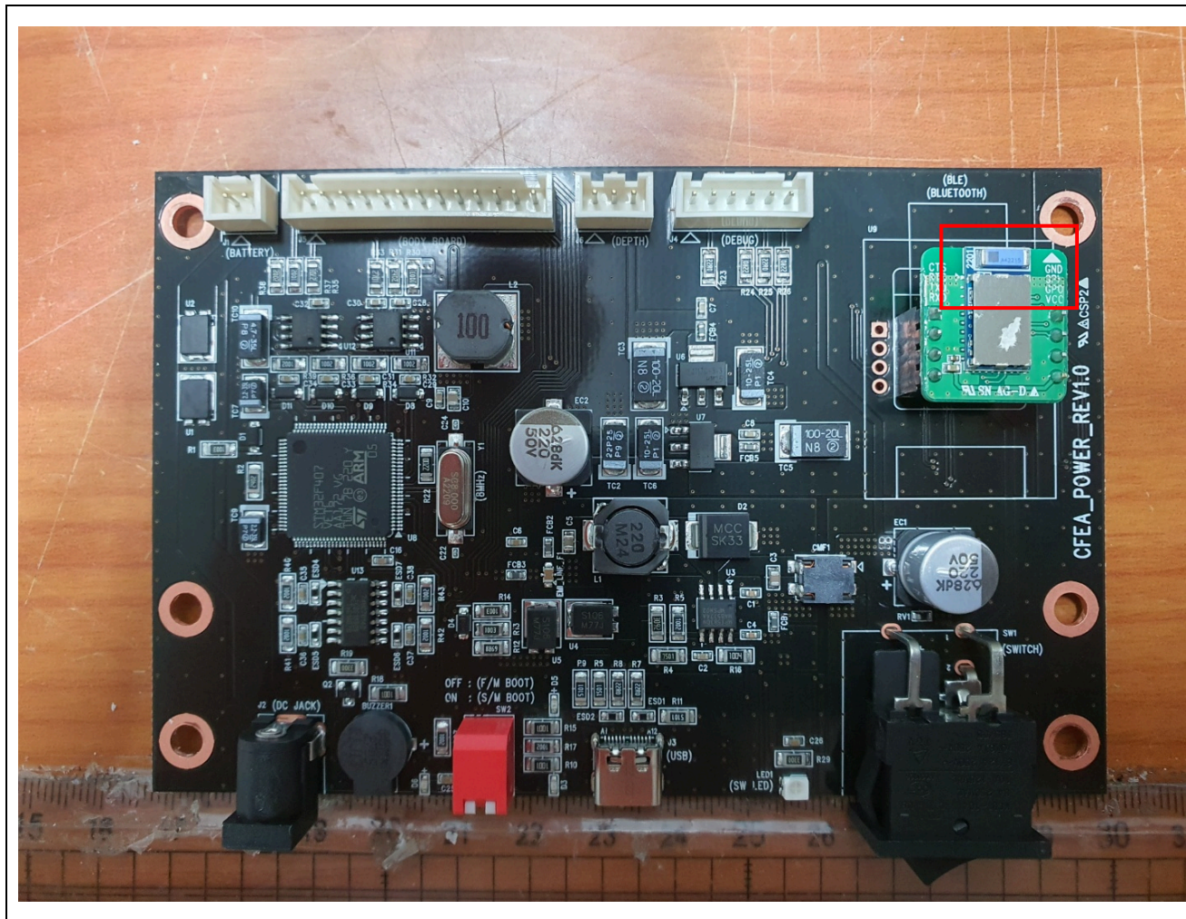
Antenna(2.4GHz ANT)
