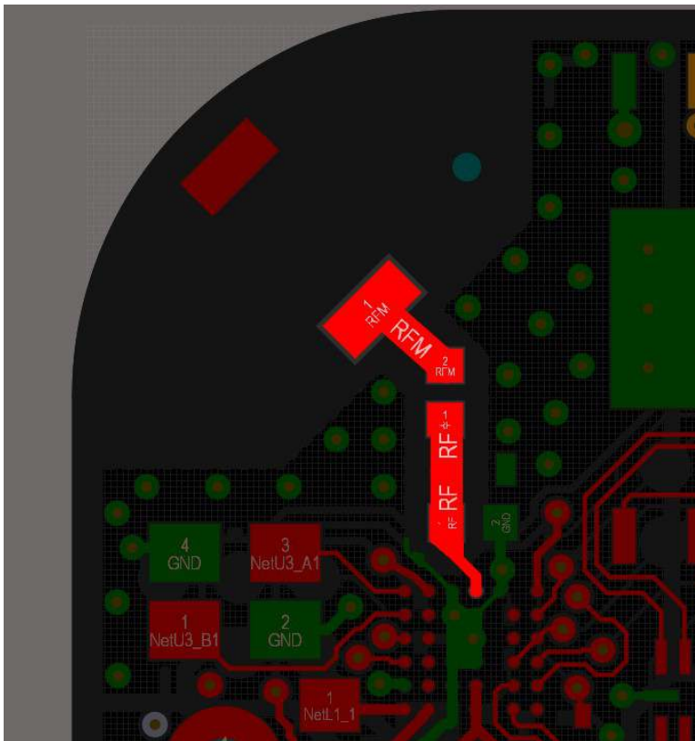
Figure 4 - Antenna Trace layout
