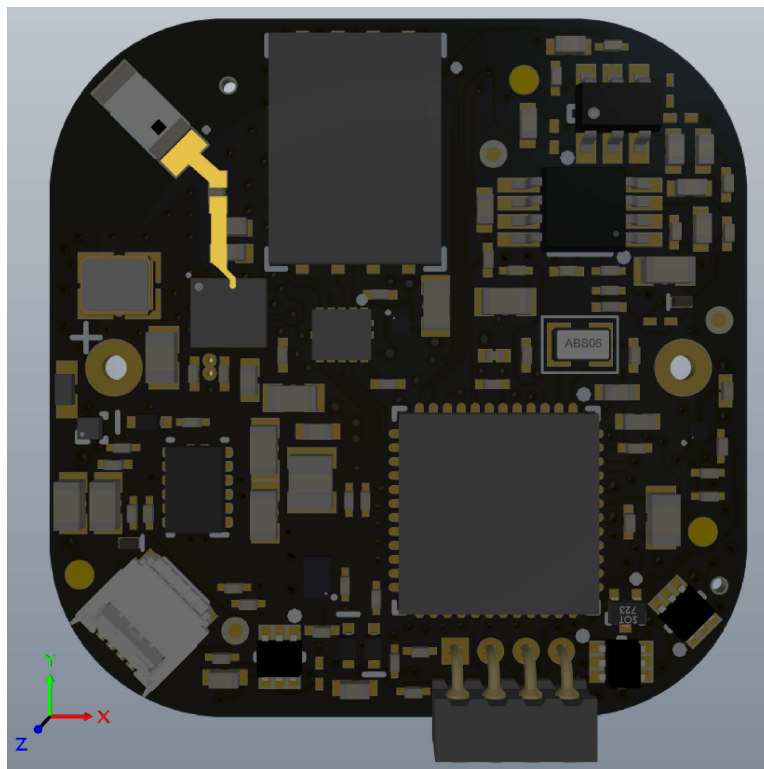
Figure 2 - View of top of PCB - Antenna highlighted
