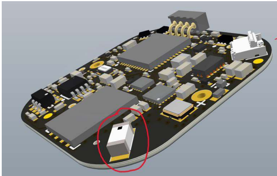
Figure 1 - Isometric view of antenna placement on PCB
