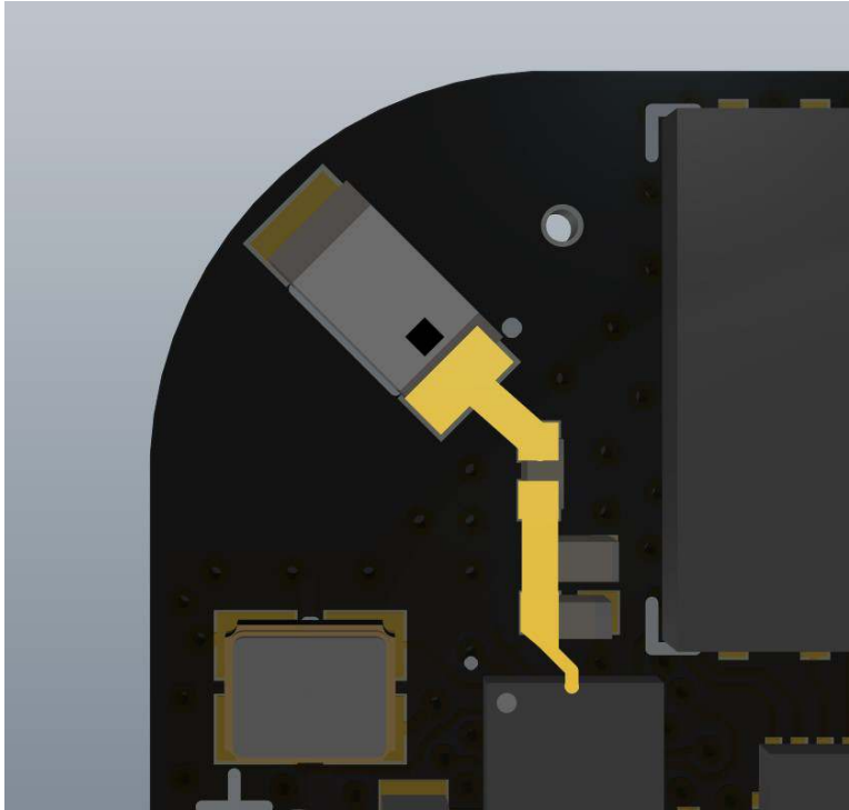
Figure 3 - Close up of antenna view
