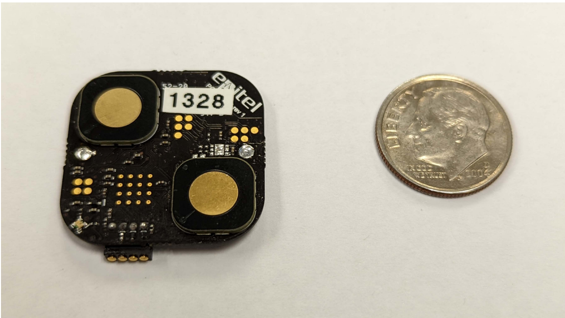
Figure 2 - PCBA - Bottom view
