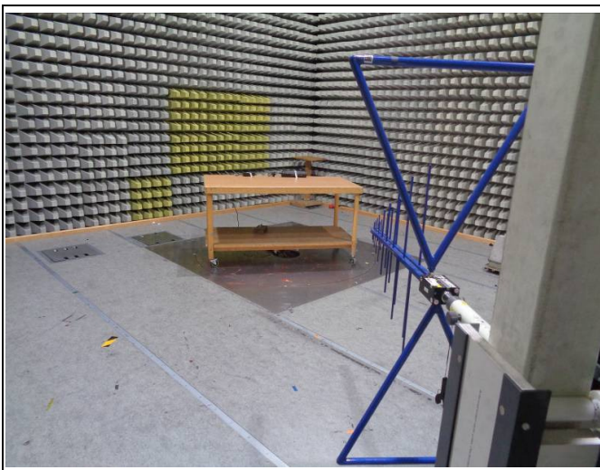
Figure 2: Test setup for radiated disturbances 30 MHz to 1000 MHz – Configuration mode 2
