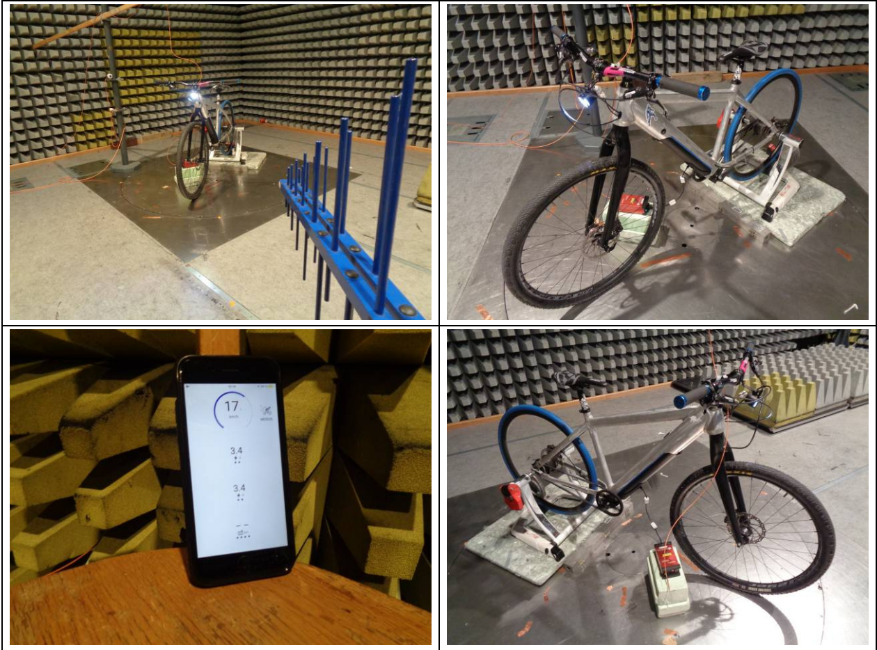
Figure 3: Test setup for radiated disturbances 30 MHz to 1000 MHz – Configuration mode 1
