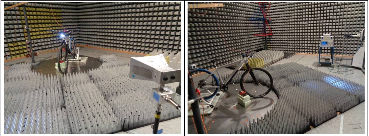
Figure 5: Test setup for radiated disturbances 18 GHz to 26 GHz – Configuration mode 1
