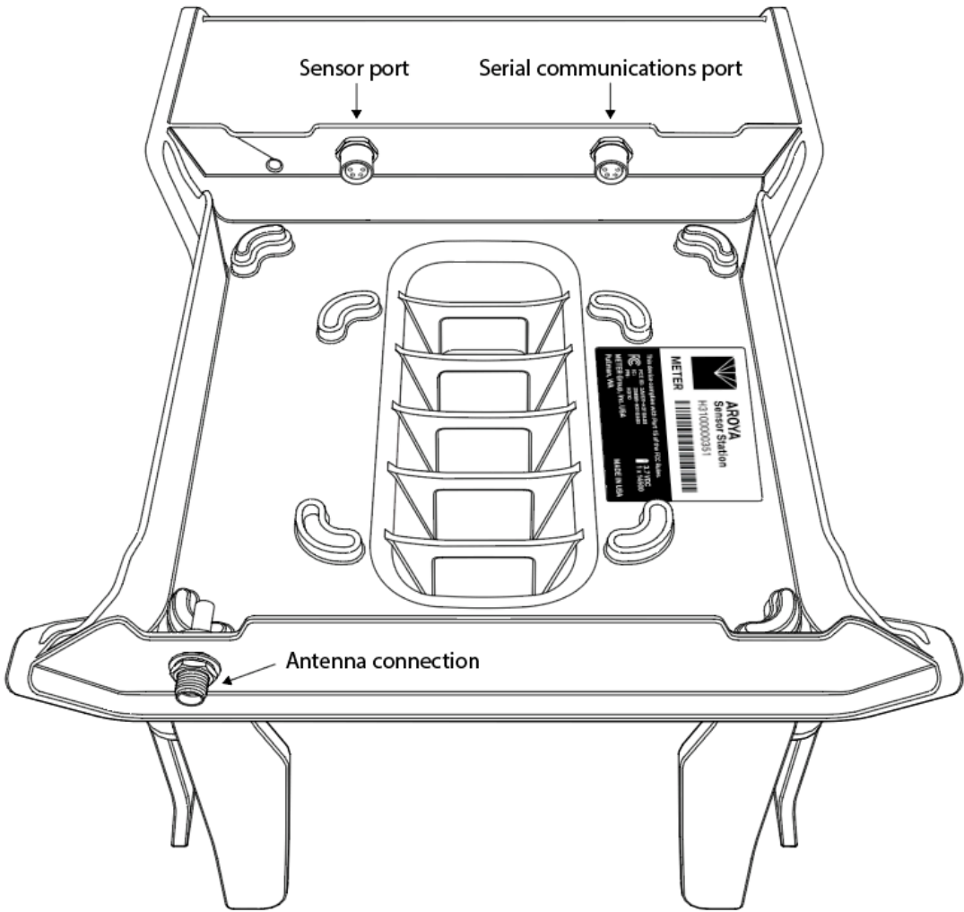
Sensor Station H3110
