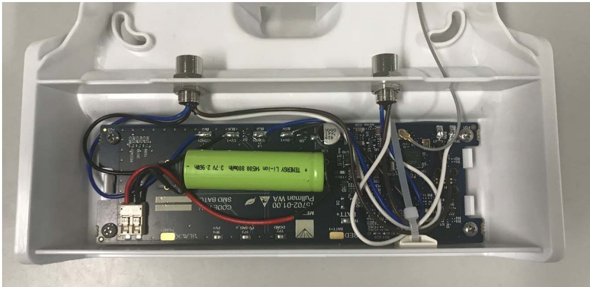
H311 Bottom View
