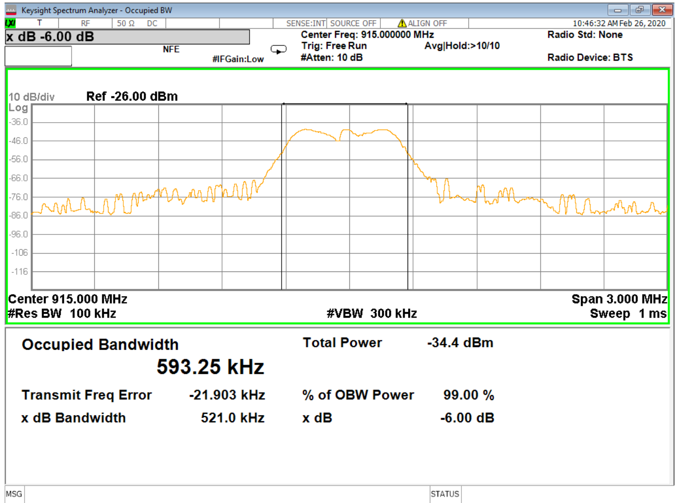
Figure 6 – Occupied Bandwidth
