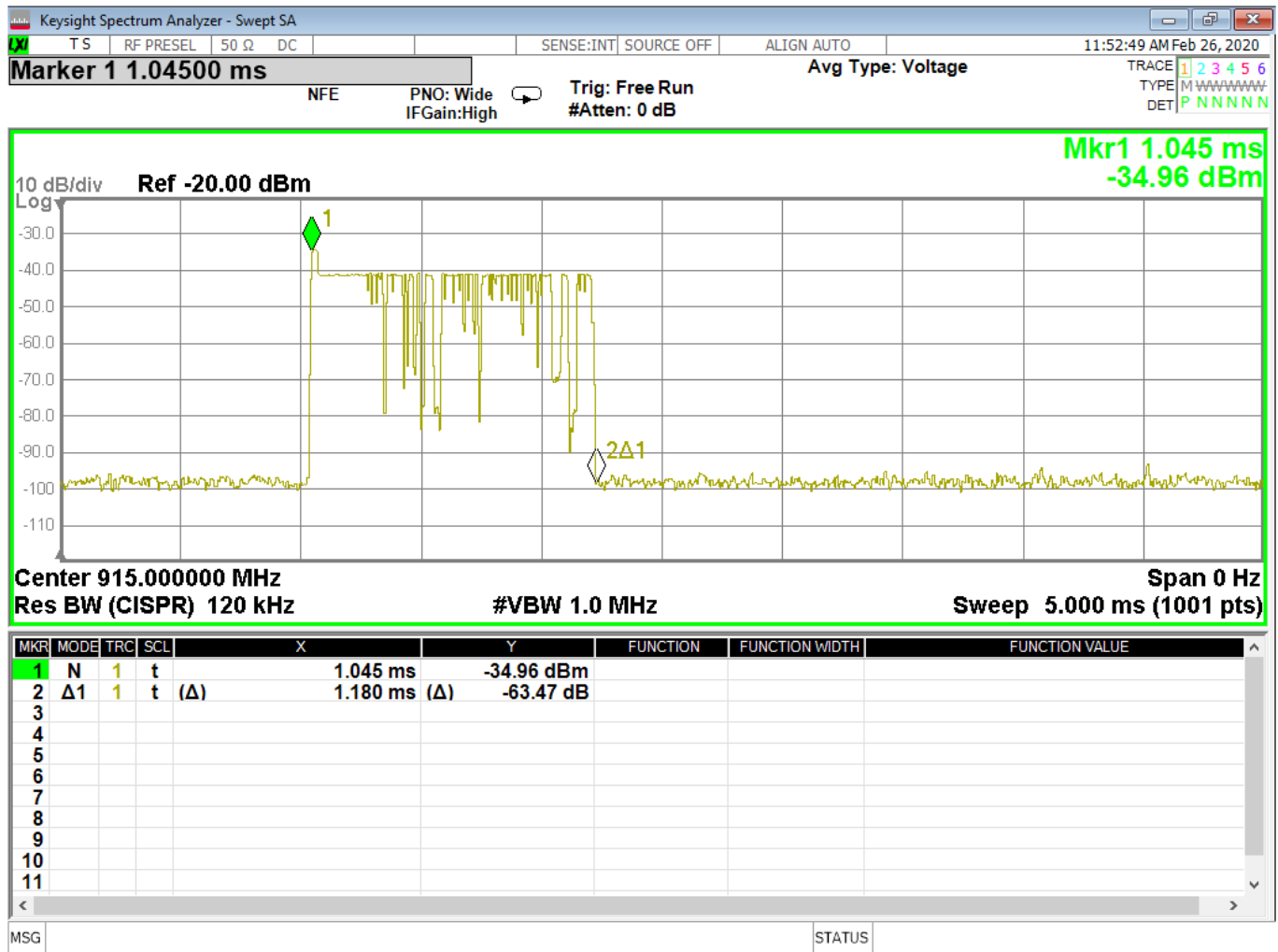
Figure 1 – ON Time
