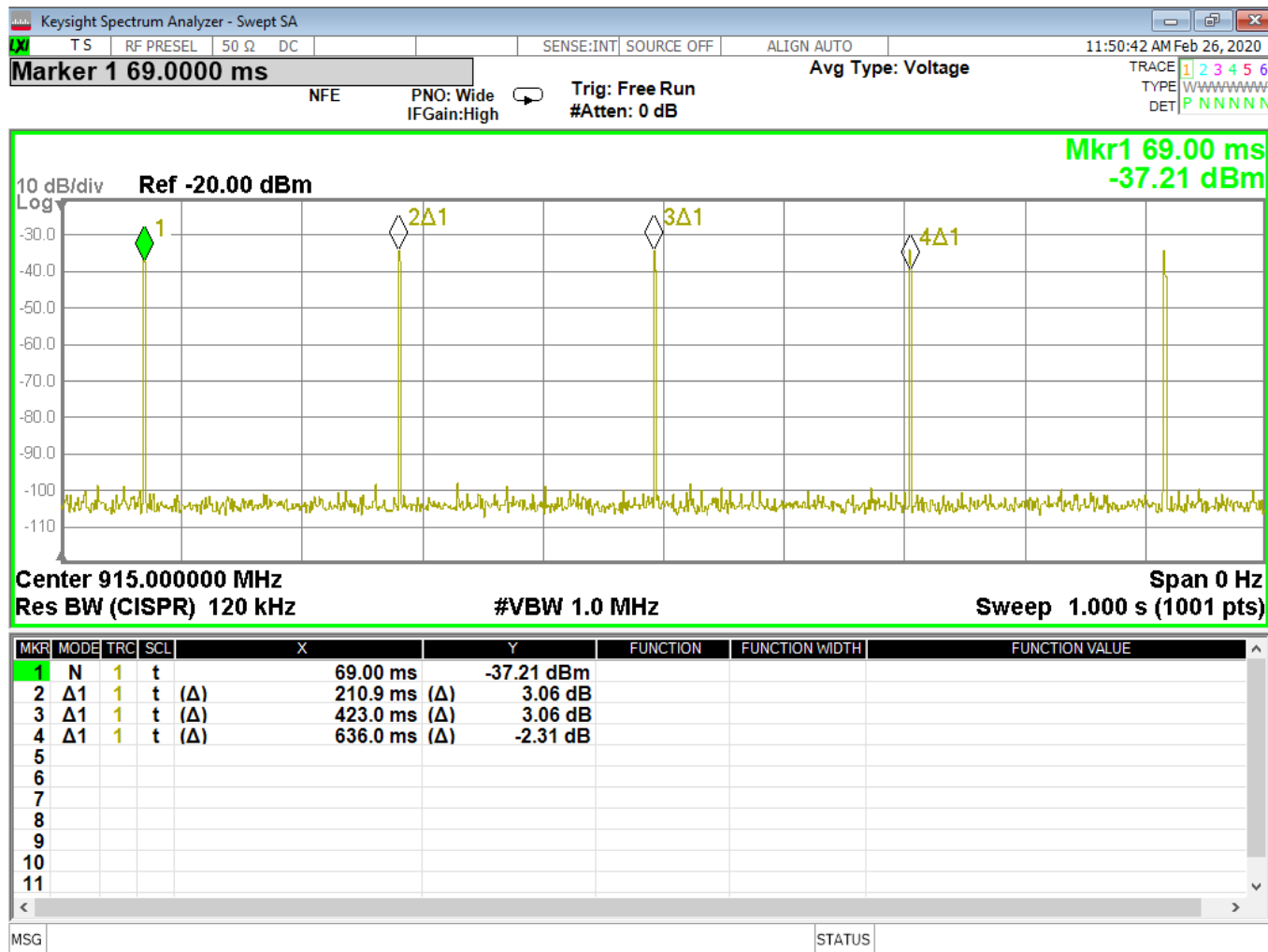
Figure 2 – Period
