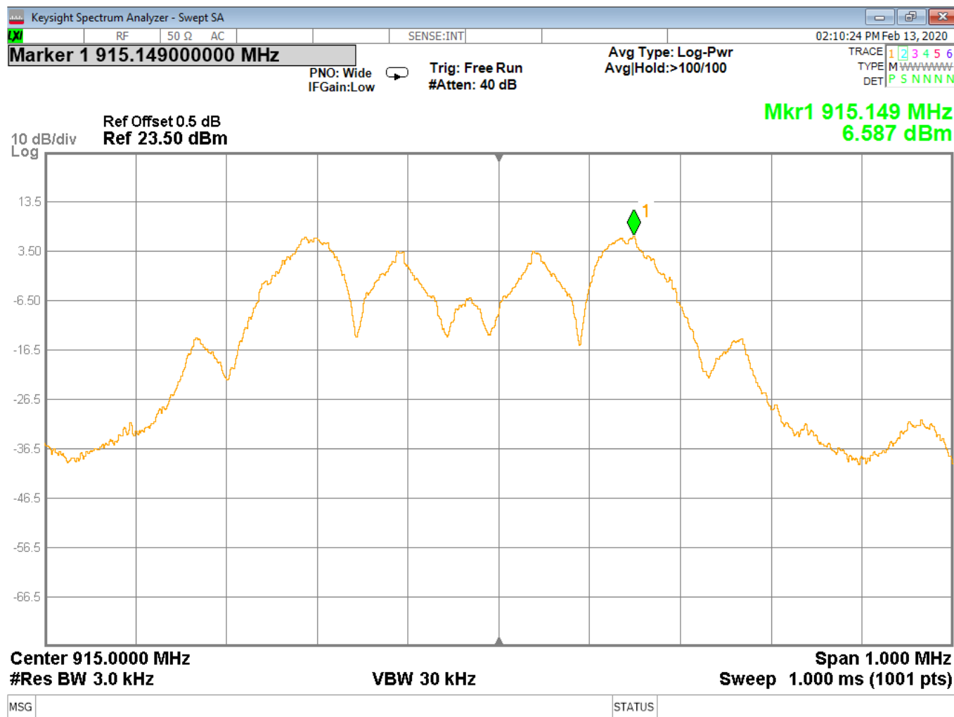
Figure 10 - Power Spectral Density
