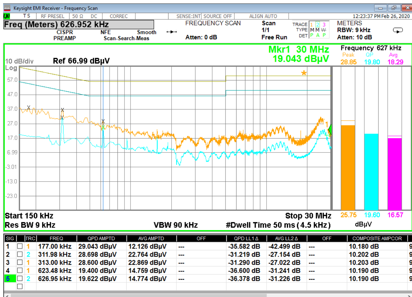
Figure 11 - Conducted Emissions, Line
