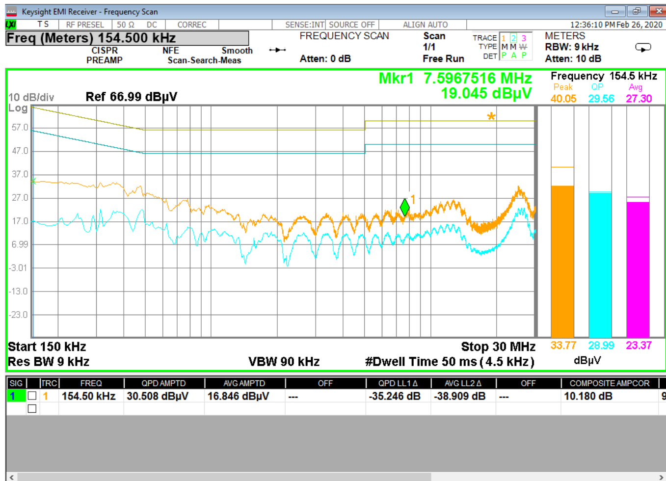
Figure 12 - Conducted Emissions, Neutral
