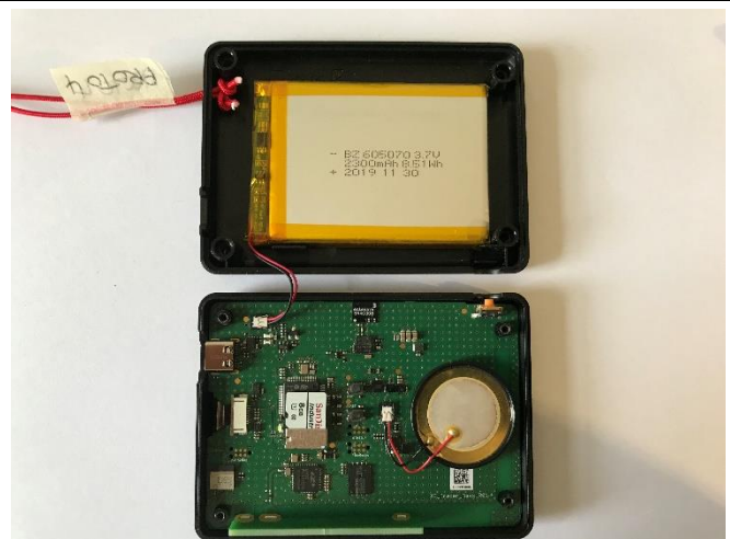
Internal view
