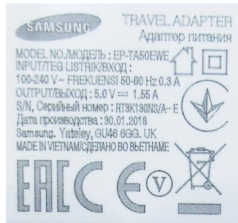
Marking on AC - USB adaptor
