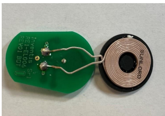
RE1-EL006 board – bottom view with coil soldered
