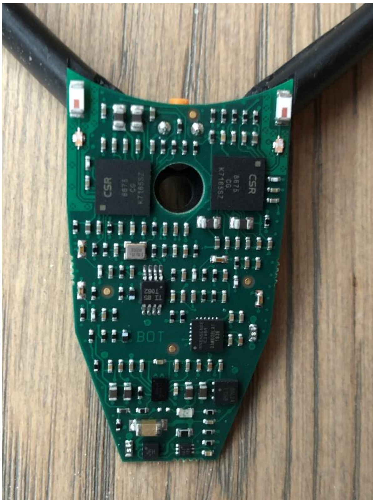
RE1-EL007 board – bottom view RE1-EL009 board – bottom view (for components reference, please refer to the appendix)
