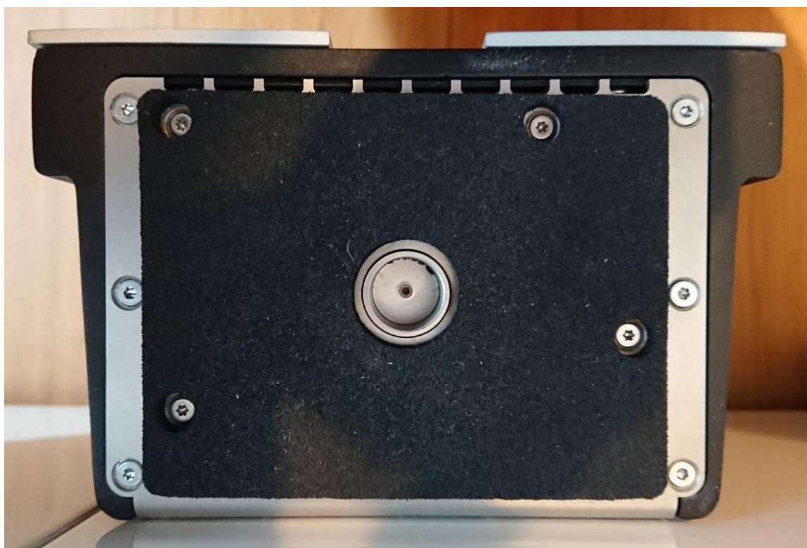
Trumpet – bottom view
