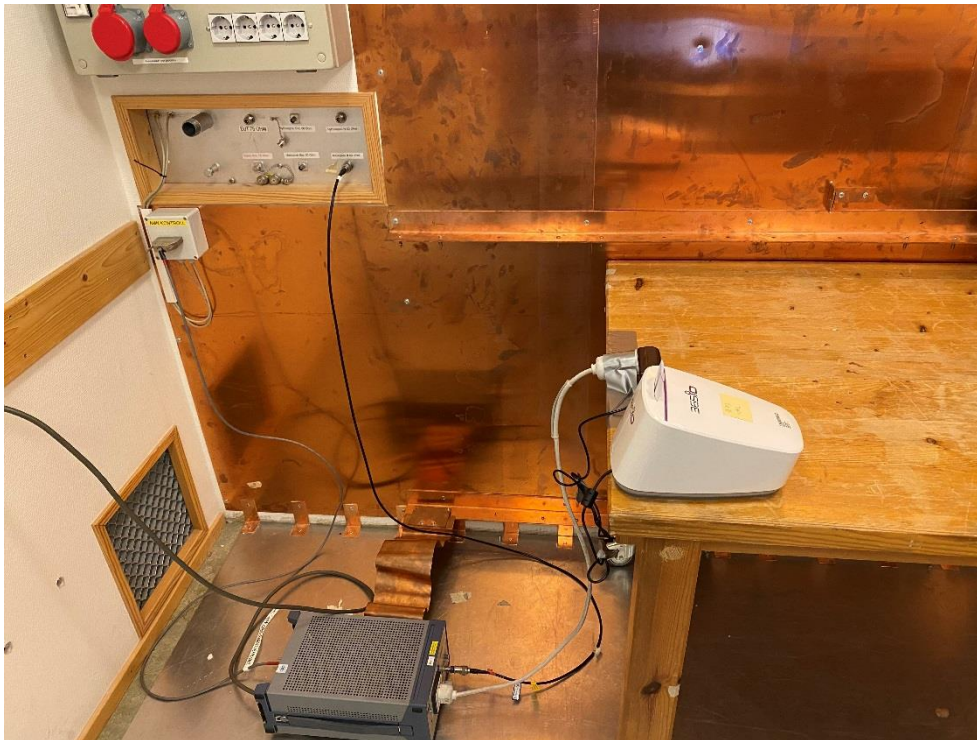
Test setup for conducted emission 150 kHz – 30 MHz
