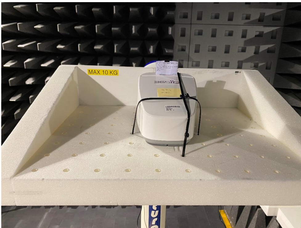
EUT position radiated emission above 1 GHz
