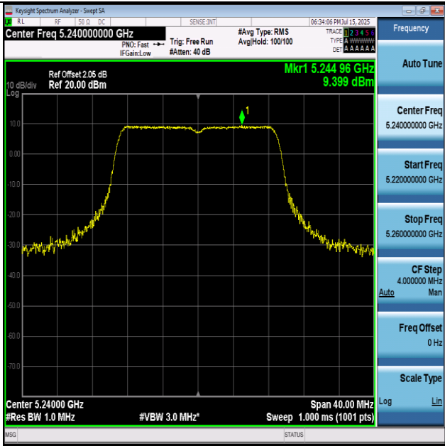
11N20-5240-PASS
