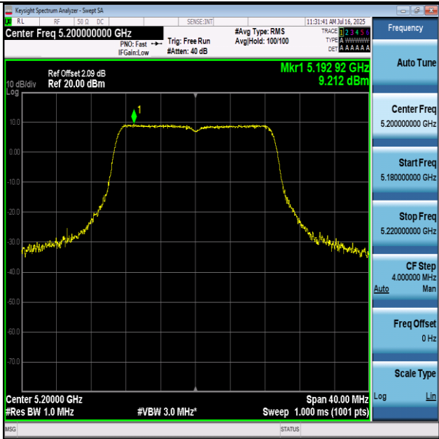
11AC20-5200-PASS
