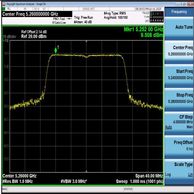
11AX20-5260-PASS
