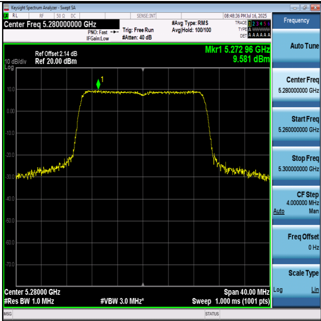
11AX20-5280-PASS
