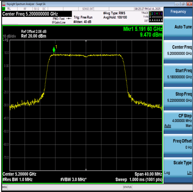
11AX20-5200-PASS
