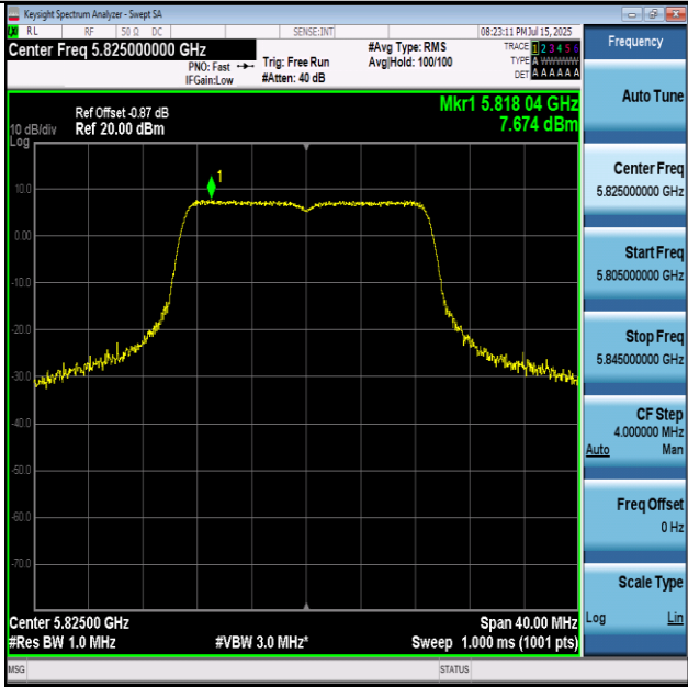
11N20-5825-PASS
