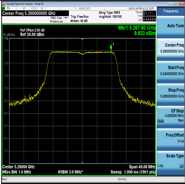
11N20-5260-PASS
