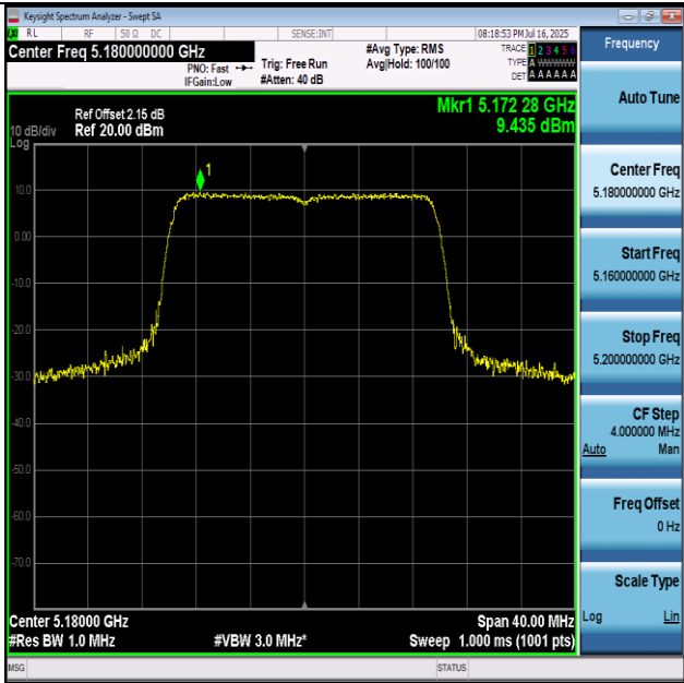
11AX20-5180-PASS
