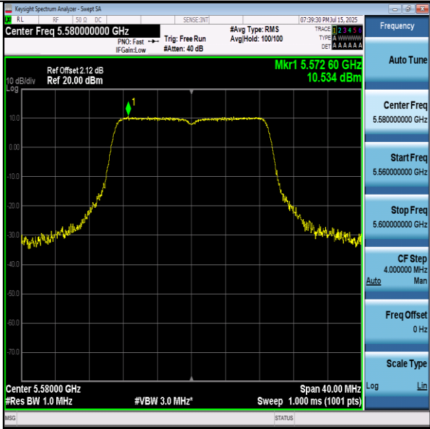
11N20-5580-PASS
