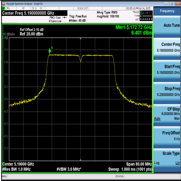
11AC40-5190-PASS
