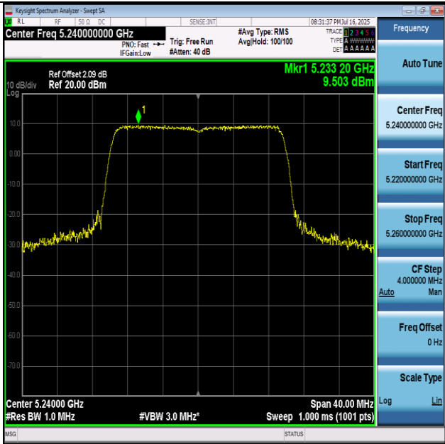
11AX20-5240-PASS
