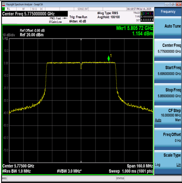
11AC80-5775-PASS
