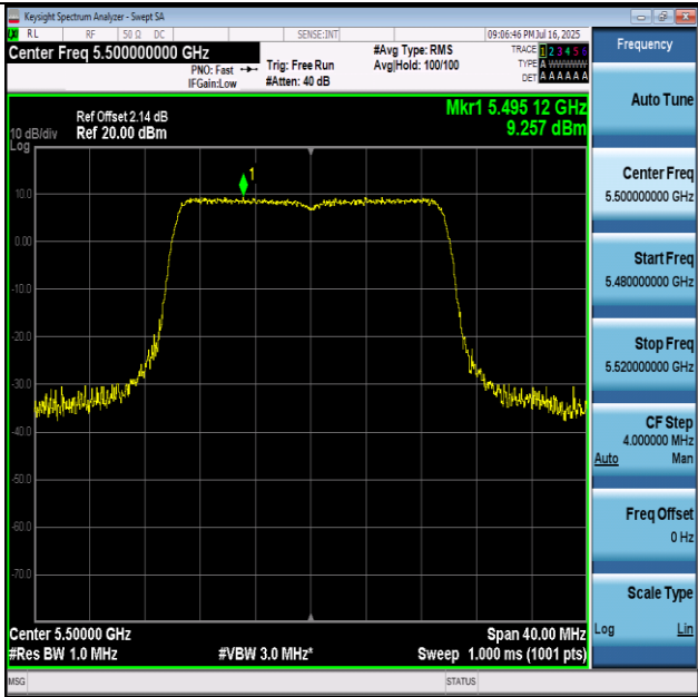
11AX20-5500-PASS
