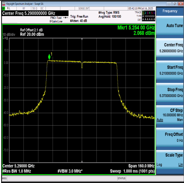
11AC80-5290-PASS
