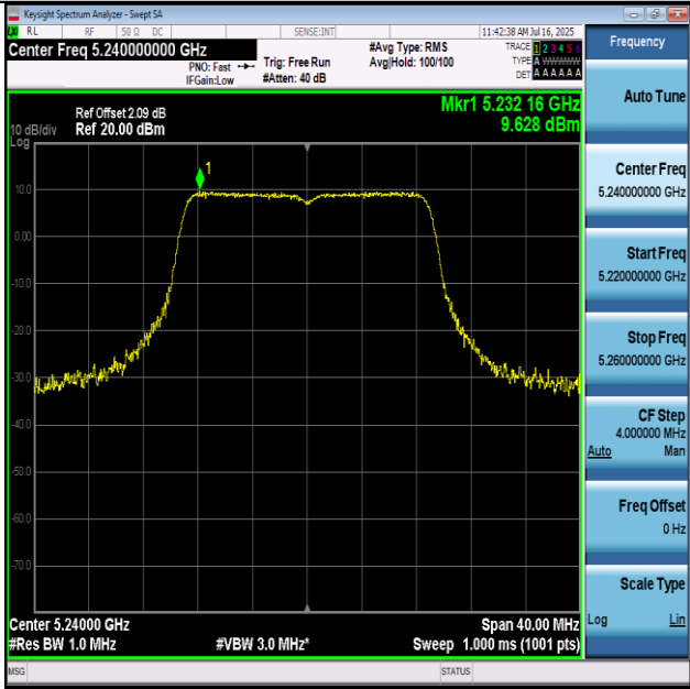
11AC20-5240-PASS
