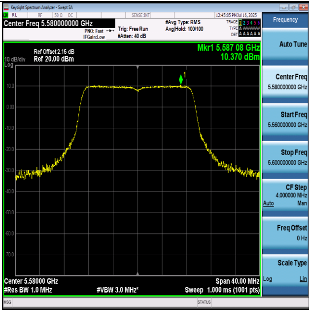
11AC20-5580-PASS
