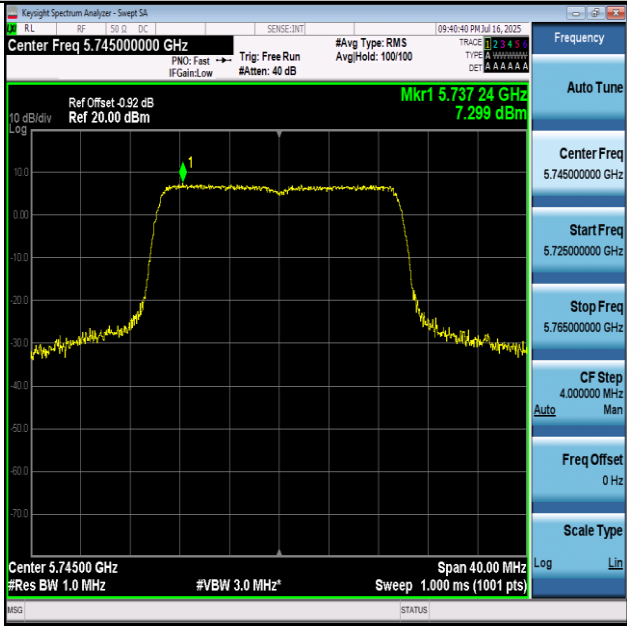
11AX20-5745-PASS
