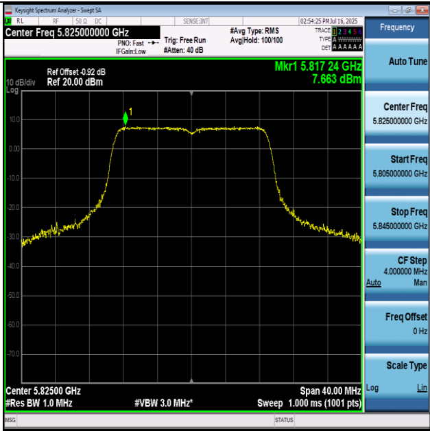
11AC20-5825-PASS
