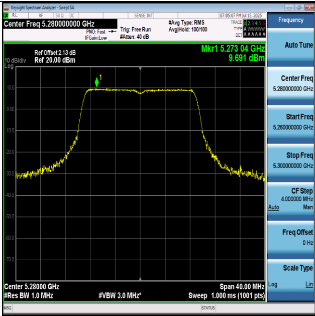
11N20-5280-PASS
