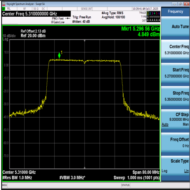
11AX40-5310-PASS
