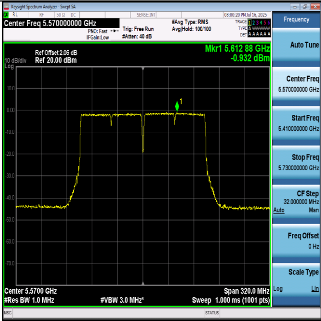
11AC160-5570-PASS
