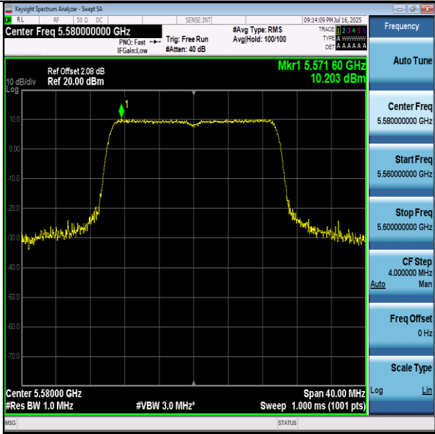
11AX20-5580-PASS
