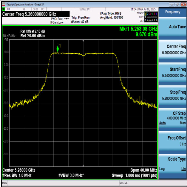
11AC20-5260-PASS
