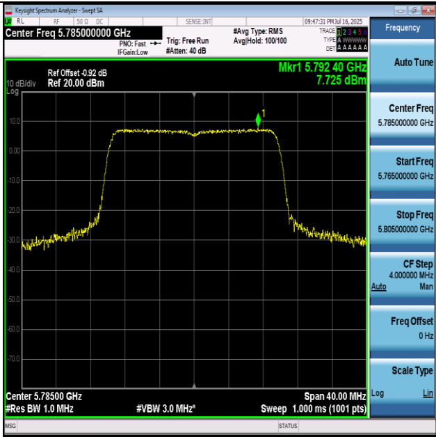
11AX20-5785-PASS
