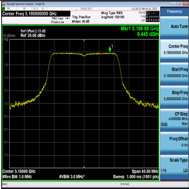
11AC20-5180-PASS
