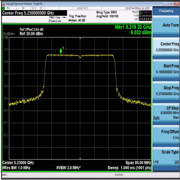
11AX40-5230-PASS
