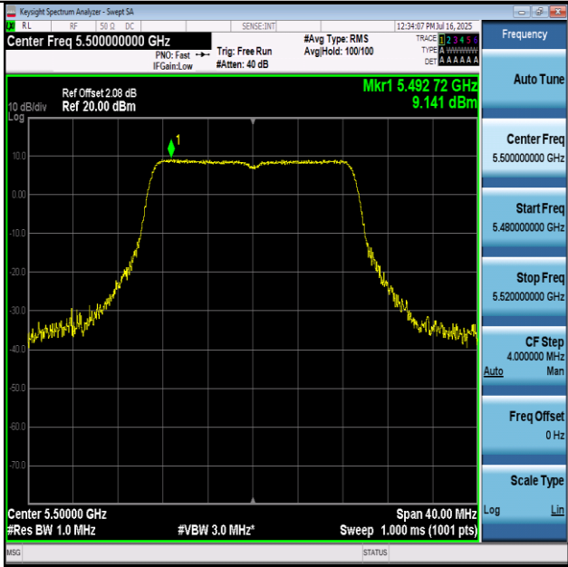
11AC20-5500-PASS
