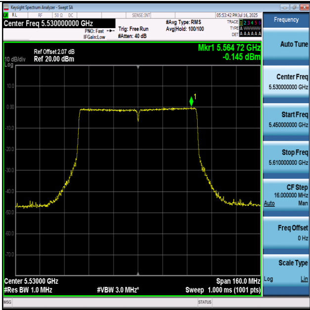
11AC80-5530-PASS
