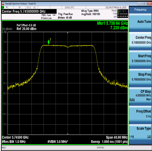
11AC20-5745-PASS
