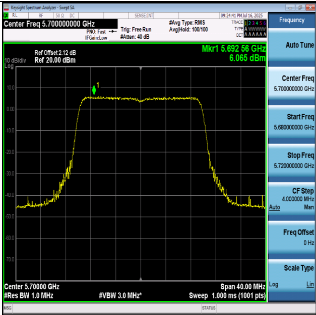
11AX20-5700-PASS
