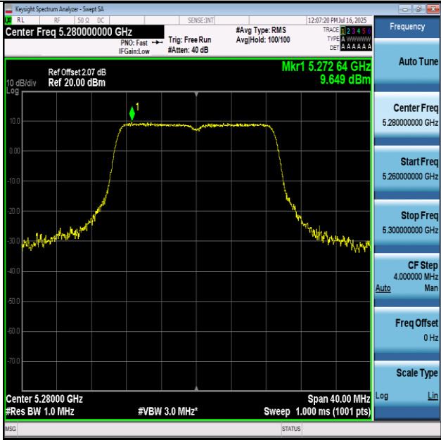
11AC20-5280-PASS
