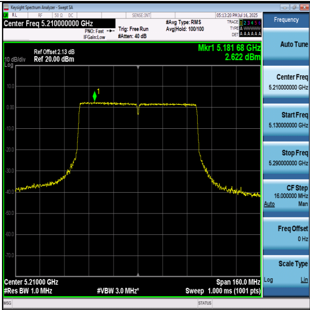
11AC80-5210-PASS
