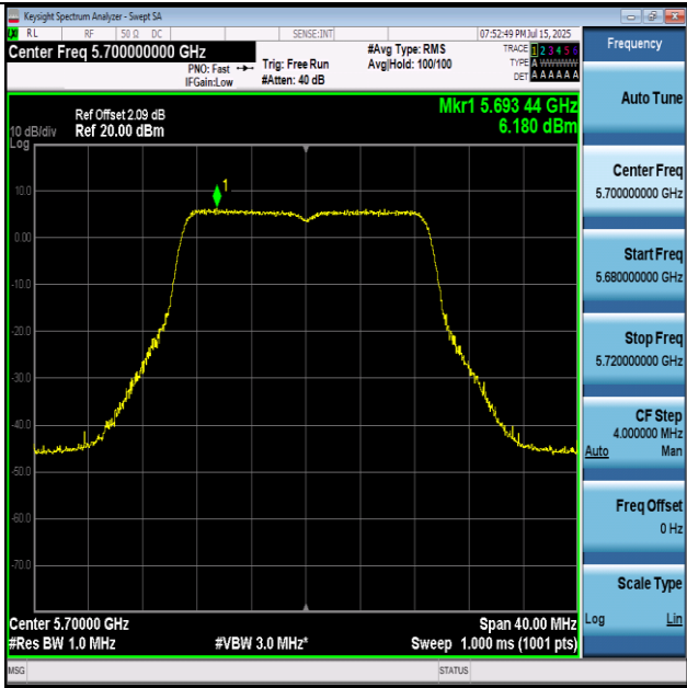
11N20-5700-PASS
