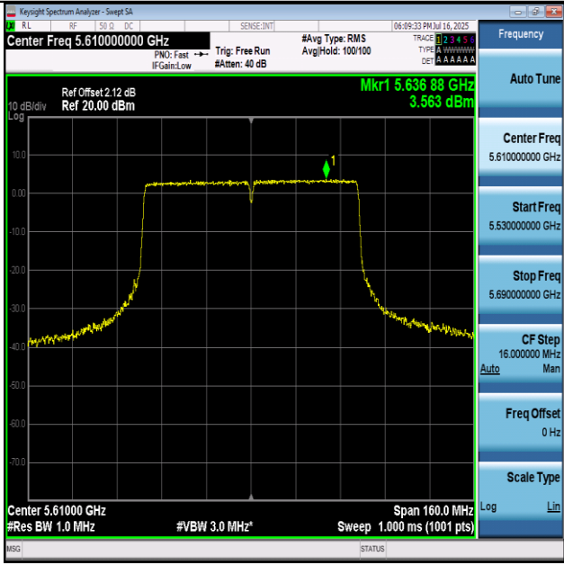
11AC80-5610-PASS
