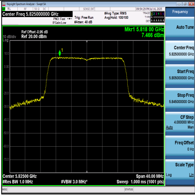
11AX20-5825-PASS
