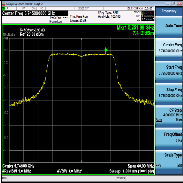
11N20-5745-PASS
