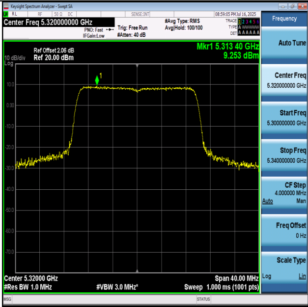
11AX20-5320-PASS
