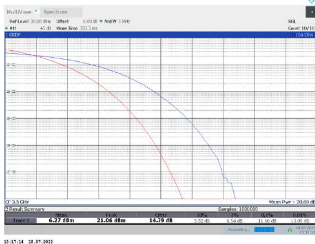
42-42-20MHz-20MHz-QPSK-QPSK-42491-42689-100RB#0-100RB#0
