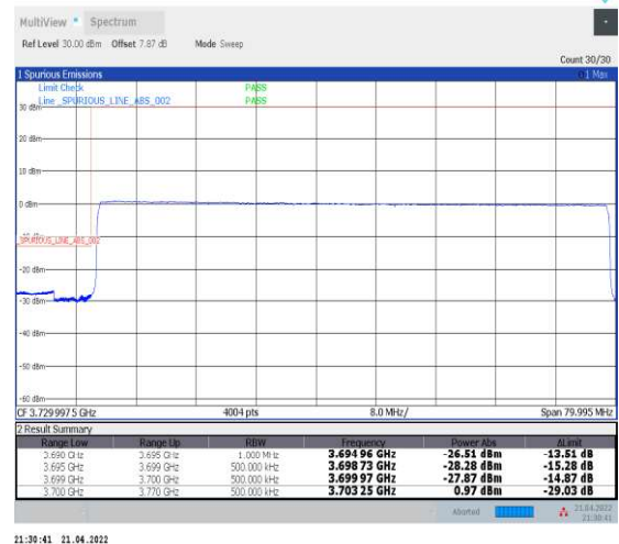
1-N78-3700-3800--30-70-L-6-CP-QPSK-Outer_Ful_I-189@0-Ant1-PASS-see graph
