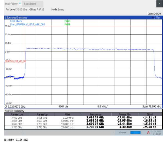
1-N78-3700-3800--30-70-L-3-DFT-PI2BPSK-Outer_Full-180@0-Ant1-PASS-see graph
