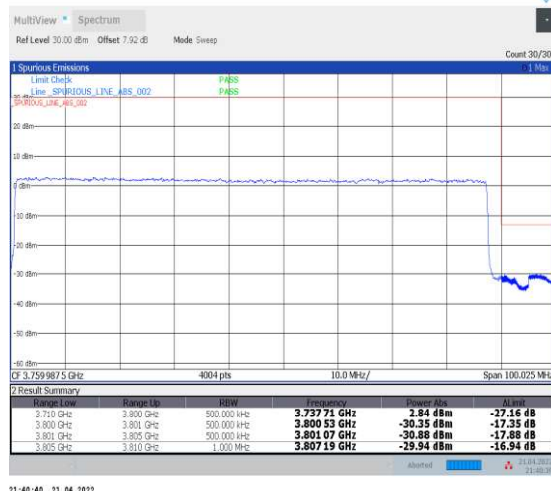
1-N78-3700-3800--30-90-H-3-DFT-PI2BPSK-Outer _Full-240@0-Ant1-PASS-see graph
