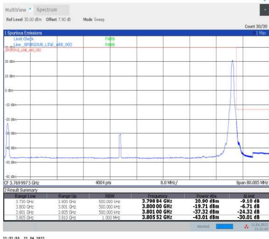
1-N78-3700-3800--30-70-H-2-DFT-PI2BPSK-Edge_1R B_Right-1@188-Ant1-PASS-see graph
