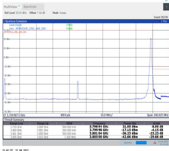
1-N78-3700-3800--30-90-H-5-CP-QPSK-Edge_1RB_R ight-1@244-Ant1-PASS-see graph
