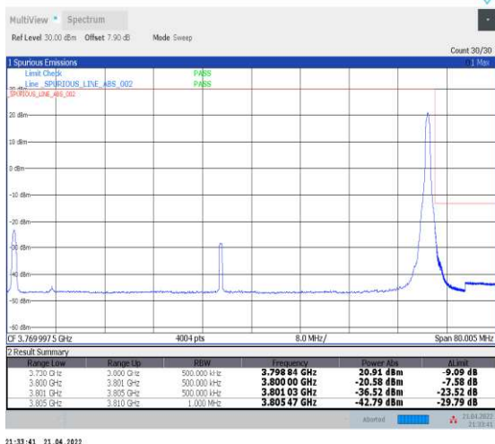
1-N78-3700-3800--30-70-H-5-CP-QPSK-Edge_1RB_R ight-1@188-Ant1-PASS-see graph
