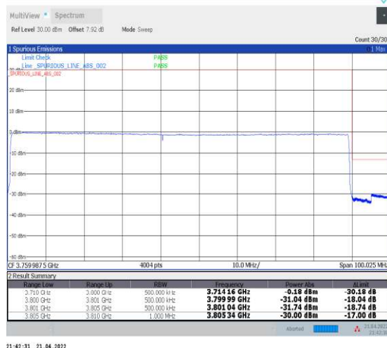
1-N78-3700-3800--30-90-H-6-CP-QPSK-Outer_Fu ll-245@0-Ant1-PASS-see graph
