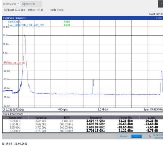
1-N78-3700-3800--30-70-L-1-DFT-PI2BPSK-Edge_1R_B_Left-1@0-Ant1-PASS-see graph
