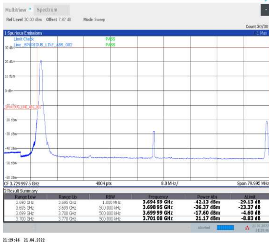
1-N78-3700-3800--30-70-L-4-CP-QPSK-Edge_1RB_L_eff-1@0-Ant1-PASS-see graph
