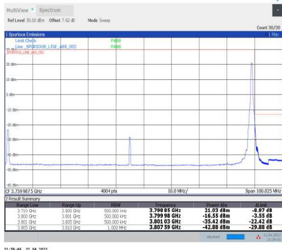
1-N78-3700-3800--30-90-H-2-DFT-PI2BPSK-Edge_1R B_Right-1@244-Ant1-PASS-see graph
