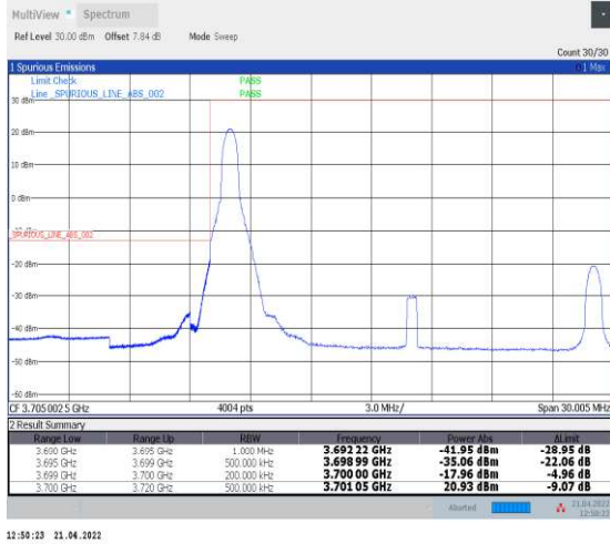
1-N78-3700-3800--30-20-L-1-DFT-PI2BPSK-Edge_1R B_Left-1@0-Ant1-PASS-see graph
