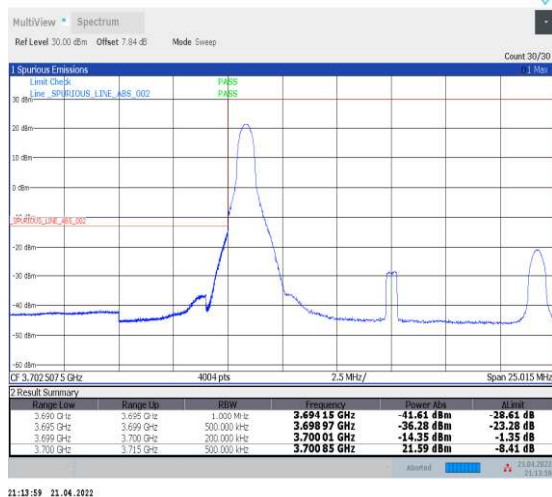
1-N78-3700-3800--30-15-L-4-CP-QPSK-Edge_1RB_L eft-1@0-Ant1-PASS-see graph
