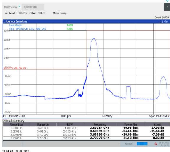
1-N78-3700-3800--30-10-L-1-DFT-PI2BPSK-Edge_1R_B_Left-1@0-Ant1-PASS-see graph
