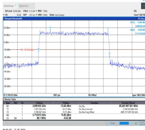
1-N78-3700-3800-PC1-30-90-L-3-DFT-16QAM-Out er_Full-240@0-Ant1-85.602-89.100-≤90-PASS
