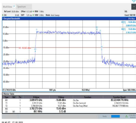
1-N78-3700-3800-PC1-30-90-L-4-DFT-64QAM-Outer_Full-240@0-Ant1-85.523-89.100-≤90-PASS
