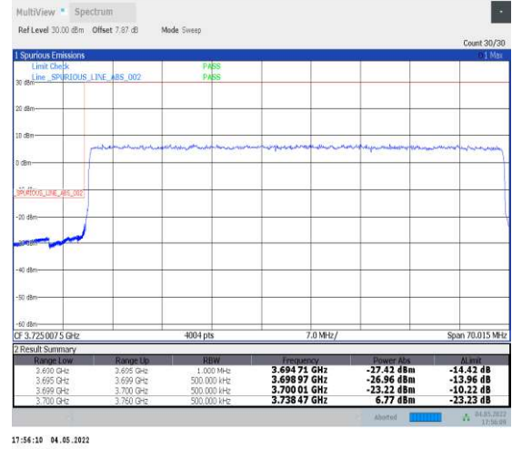
1-N78-3700-3800--30-60-L-3-DFT-PI2BPSK-Outer _Full-162@0-Ant1-PASS-see graph
