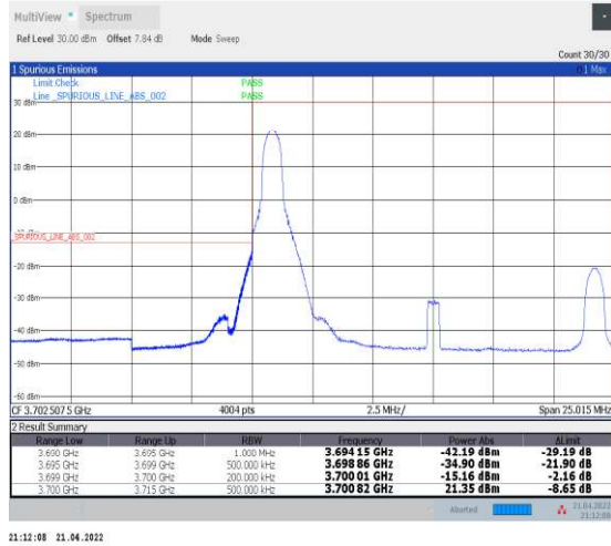
1-N78-3700-3800--30-15-L-1-DFT-PI2BPSK-Edge_1R B_Left-1@0-Ant1-PASS-see graph
