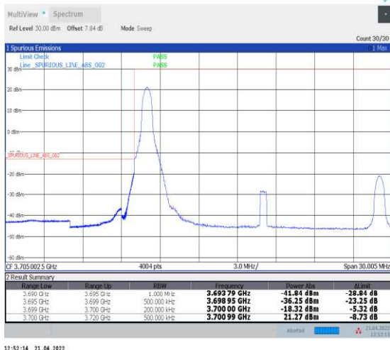
1-N78-3700-3800--30-20-L-4-CP-QPSK-Edge_1RB_L eft-1@0-Ant1-PASS-see graph
