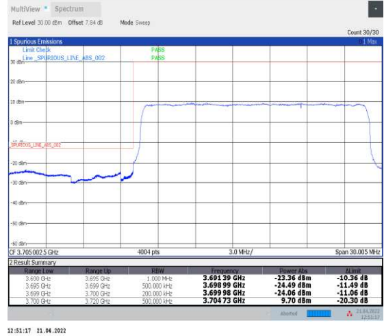
1-N78-3700-3800--30-20-L-3-DFT-PI2BPSK-Outer _Full-50@0-Ant1-PASS-see graph
