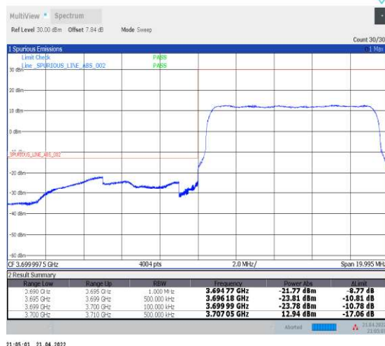
1-N78-3700-3800--30-10-L-3-DFT-PI2BPSK-Outer_Full-24@0-Ant1-PASS-see graph
