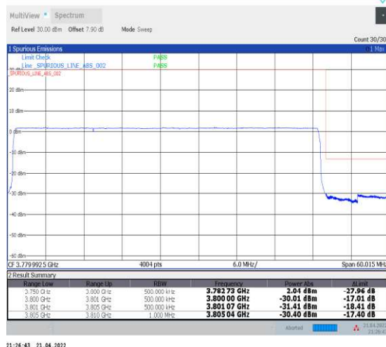
1-N78-3700-3800--30-50-H-6-CP-QPSK-Outer_Fu ll-133@0-Ant1-PASS-see graph
