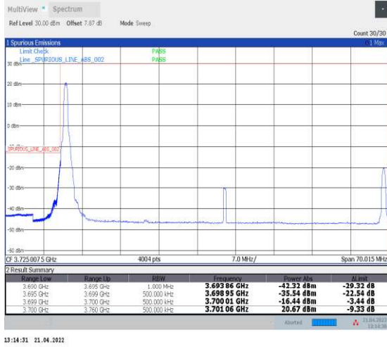
1-N78-3700-3800--30-60-L-1-DFT-PI2BPSK-Edge_1R B_Left-1@0-Ant1-PASS-see graph
