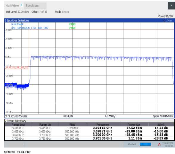
1-N78-3700-3800--30-60-L-6-CP-QPSK-Outer_Ful I-162@0-Ant1-PASS-see graph
