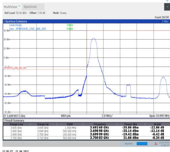
1-N78-3700-3800--30-10-L-4-CP-QPSK-Edge_1RB_L_eff-1@0-Ant1-PASS-see graph
