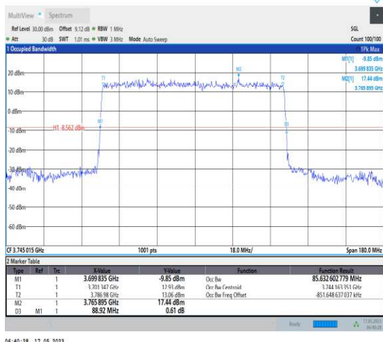
1-N78-3700-3800-PC1-30-90-L-2-DFT-PI2BPSK-Out er_Full-240@0-Ant1-85.633-88.920-≤90-PASS
