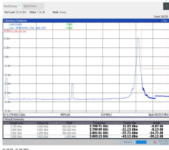
1-N78-3700-3800--30-50-H-2-DFT-PI2BPSK-Edge_1R B_Right-1@132-Ant1-PASS-see graph
