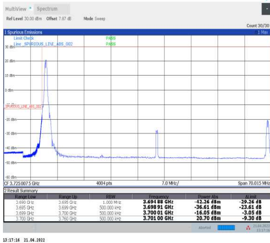
1-N78-3700-3800--30-60-L-4-CP-QPSK-Edge_1RB_L eft-1@0-Ant1-PASS-see graph
