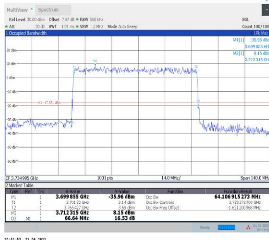
1-N78-3700-3800--30-70-L-5-DFT-256QAM-Out_F ull-180@0-Ant1-64.107-66.640-≤70-PASS
