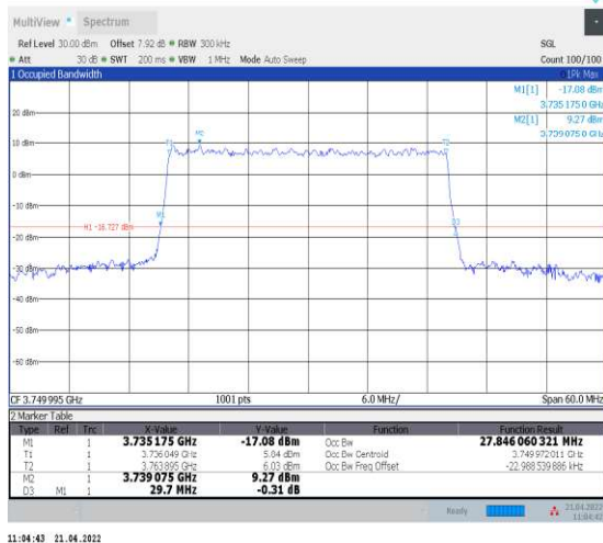
1-N78-3700-3800--30-30-M-9-CP-256QAM-Outer_F ull-78@0-Ant1-27.846-29.700-≤30-PASS
