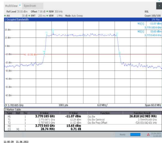
1-N78-3700-3800--30-30-H-1-DFT-QPSK-Outer_Full -75@0-Ant1-26.818-28.740-≤30-PASS
