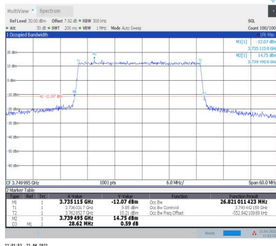
1-N78-3700-3800--30-30-M-4-DFT-64QAM-Outer_F ull-75@0-Ant1-26.821-28.620-≤30-PASS
