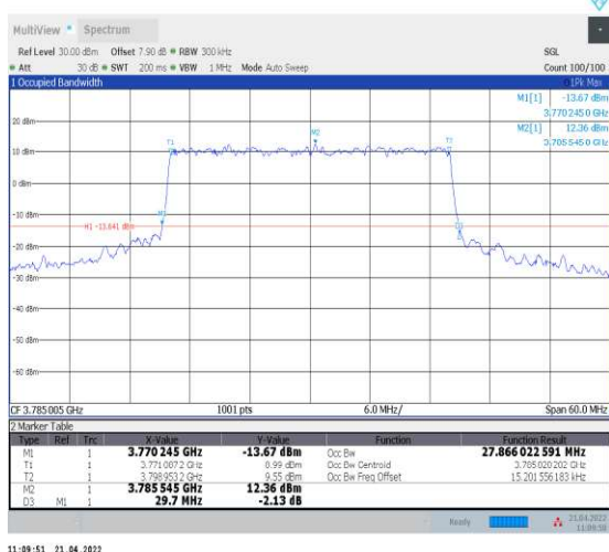
1-N78-3700-3800--30-30-H-8-CP-64QAM-Outer_Full-78@0-Ant1-27.866-29.700-≤30-PASS
