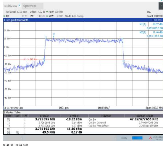
1-N78-3700-3800--30-50-M-8-CP-64QAM-Outer_Ful I-133@0-Ant1-47.558-49.500-≤50-PASS
