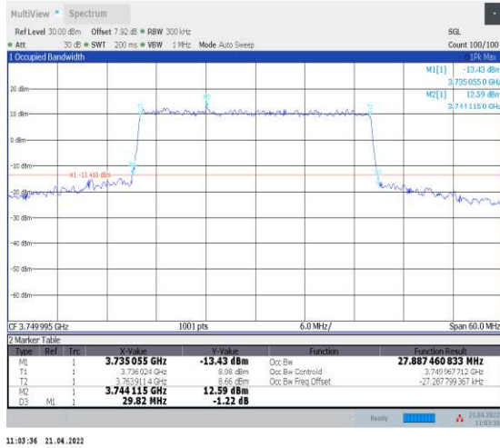
1-N78-3700-3800--30-30-M-7-CP-16QAM-Outer_Full -78@0-Ant1-27.887-29.820-≤30-PASS
