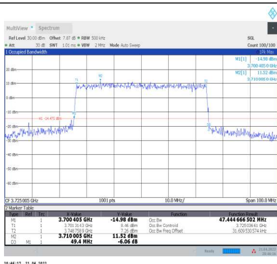
1-N78-3700-3800--30-50-L-6-CP-QPSK-Outer_Full-1 33@0-Ant1-47.445-49.400-≤50-PASS
