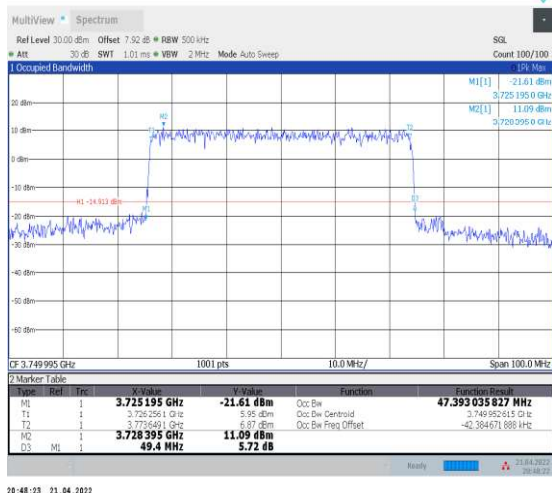
1-N78-3700-3800--30-50-M-7-CP-16QAM-Outer_Full -133@0-Ant1-47.393-49.400-≤50-PASS
