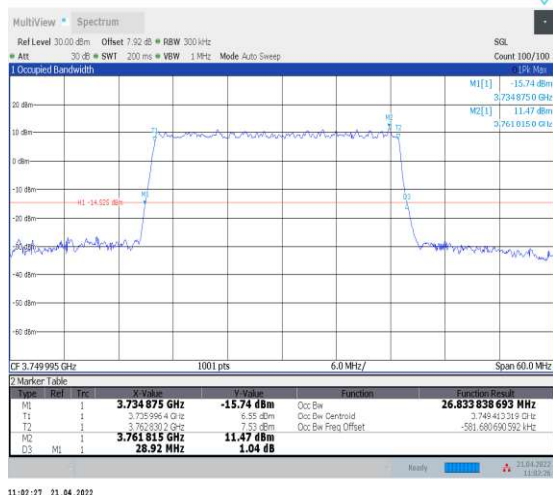
1-N78-3700-3800--30-30-M-5-DFT-256QAM-Outer_ Full-75@0-Ant1-26.834-28.920-≤30-PASS
