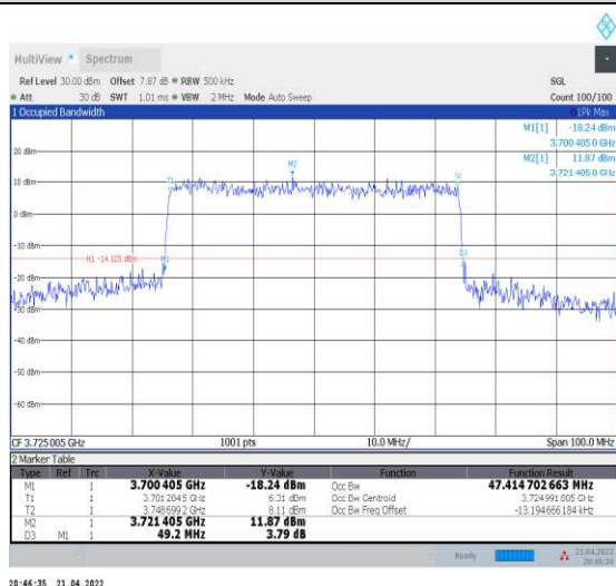
1-N78-3700-3800--30-50-L-8-CP-64QAM-Outer_Full -133@0-Ant1-47.415-49.200-≤50-PASS
