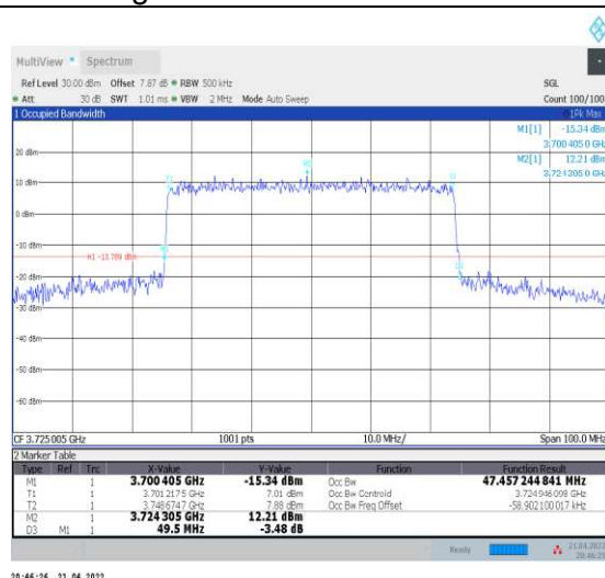
1-N78-3700-3800--30-50-L-7-CP-16QAM-Outer_Full -133@0-Ant1-47.457-49.500-≤50-PASS
