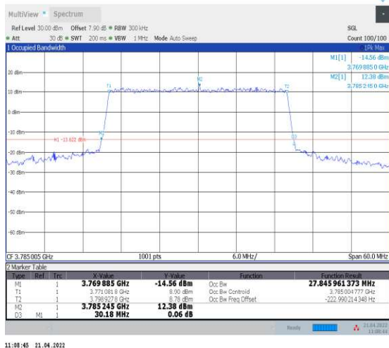
1-N78-3700-3800--30-30-H-6-CP-QPSK-Outer_Full-78@0-Ant1-27.846-30.180-≤30-PASS
