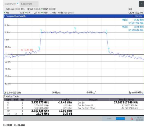
1-N78-3700-3800--30-30-M-8-CP-64QAM-Outer_Ful I-78@0-Ant1-27.868-29.760-≤30-PASS
