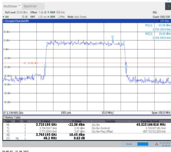
1-N78-3700-3800--30-50-M-5-DFT-256QAM-Outer_ Full-128@0-Ant1-45.525-48.200-≤50-PASS
