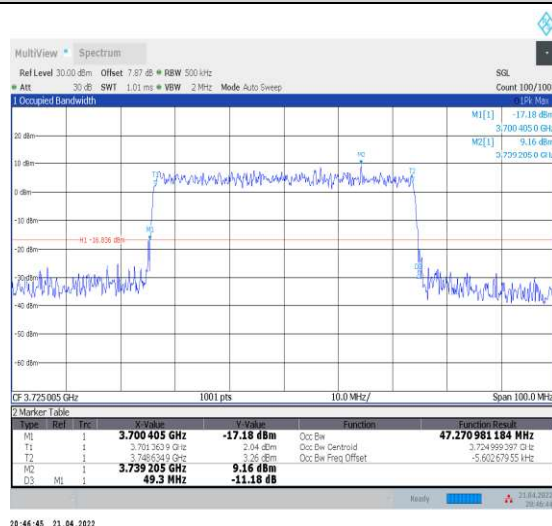
1-N78-3700-3800--30-50-L-9-CP-256QAM-Outer_Fu ll-133@0-Ant1-47.271-49.300-≤50-PASS
