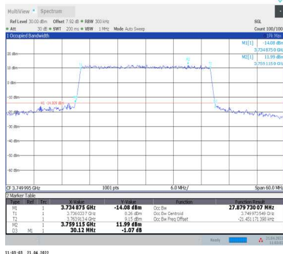
1-N78-3700-3800--30-30-M-6-CP-QPSK-Outer_Full- 78@0-Ant1-27.88-30.120-≤30-PASS
