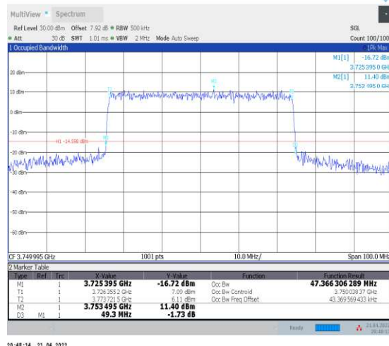
1-N78-3700-3800--30-50-M-6-CP-QPSK-Outer_Full- 133@0-Ant1-47.366-49.300-≤50-PASS
