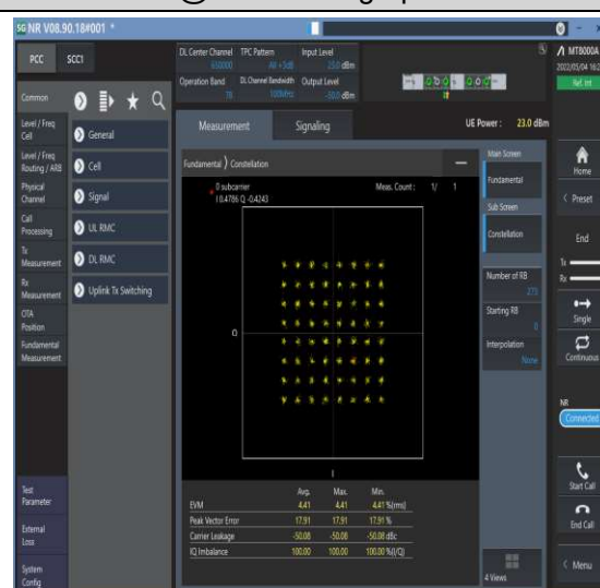
1-N78-3700-3800--30-100-M-8-CP-64QAM-Out-er_Fu Full-270@0-Ant1-see graph-PASS
