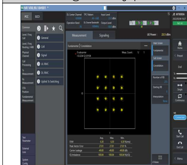
1-N78-3700-3800--30-100-M-7-CP-16QAM-Out-er_Fu Full-270@0-Ant1-see graph-PASS
