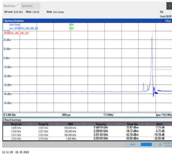
1-N78-3450-3550-PC1-30-10-H-5-CP-QPSK-Edge_1R_B_Right-1@23-Ant1-1--PASS-see graph
