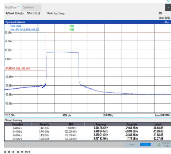
1-N78-3450-3550-PC1-30-40-L-6-CP-QPSK-Outer_Full-106@0-Ant1-1--PASS-see graph
