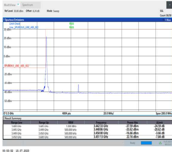
1-N78-3450-3550-PC1-30-40-L-1-DFT-PI2BPSK-Edge_1RB_Left-1@0-Ant1-1--PASS-see graph
