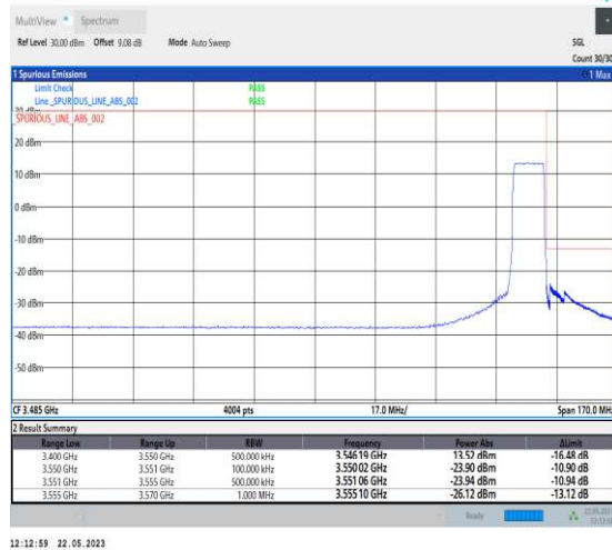
1-N78-3450-3550-PC1-30-10-H-6-CP-QPSK-Outer_Full-24@0-Ant1-1--PASS-see graph
