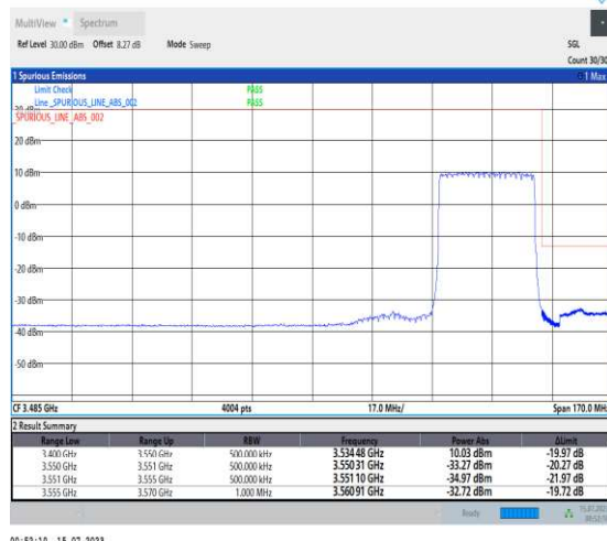
1-N78-3450-3550-PC1-30-30-H-3-DFT-PI2BPSK-Outer_Full-75@0-Ant1-1--PASS-see graph
