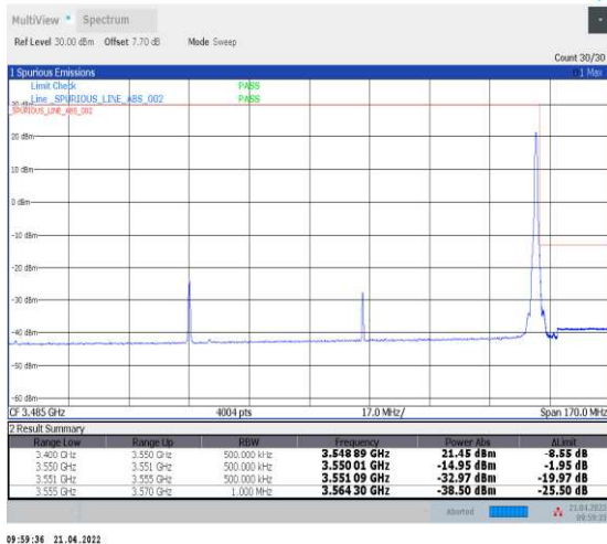
1-N78-3450-3550--30-100-H-5-CP-QPSK-Edge_1RB_Right-1@272-Ant1-PASS-see graph
