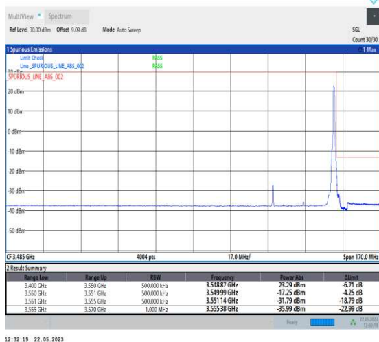
1-N78-3450-3550-PC1-30-30-H-5-CP-QPSK-Edge_1R_B_Right-1@77-Ant1-1--PASS-see graph
