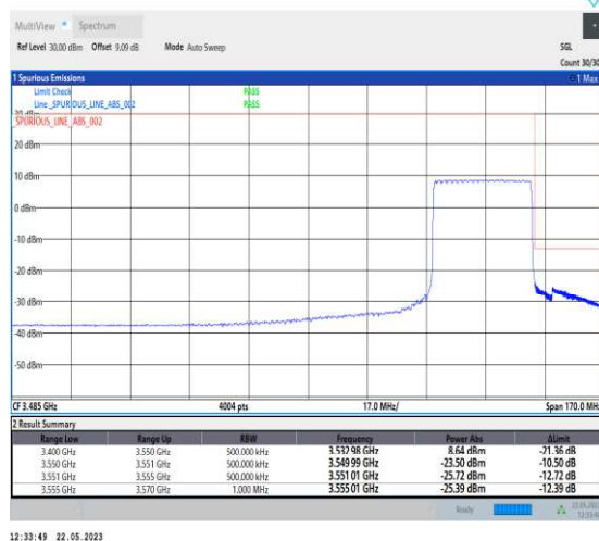
1-N78-3450-3550-PC1-30-30-H-6-CP-QPSK-Outer_Full-78@0-Ant1-1--PASS-see graph
