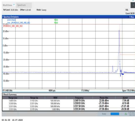
1-N78-3450-3550-PC1-30-10-H-2-DFT-PI2BPSK-Edge_1RB_Right-1@23-Ant1-1--PASS-see graph
