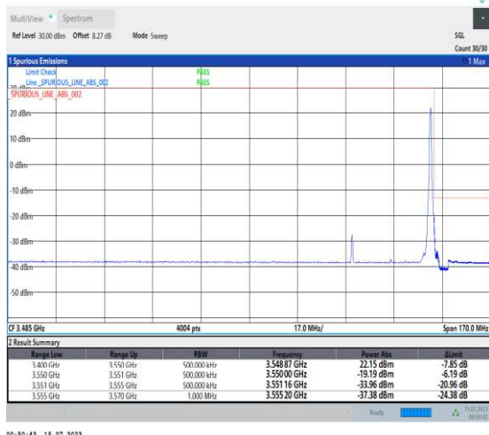
1-N78-3450-3550-PC1-30-30-H-2-DFT-PI2BPSK-Edge_1RB_Right-1@77-Ant1-1--PASS-see graph
