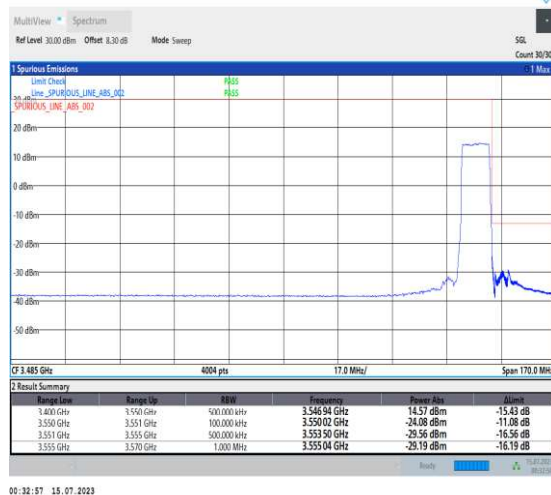
1-N78-3450-3550-PC1-30-10-H-3-DFT-PI2BPSK-Outer_Full-24@0-Ant1-1--PASS-see graph
