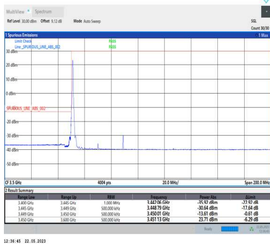
1-N78-3450-3550-PC1-30-40-L-4-CP-QPSK-Edge_1RB_Left-1@0-Ant1-1--PASS-see graph
