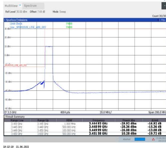
1-N78-3450-3550--30-10-L-6-CP-QPSK-Outer_Ful_I-24@0-Ant1-PASS-see graph
