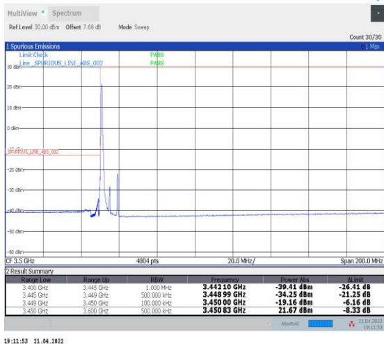
1-N78-3450-3550--30-10-L-4-CP-QPSK-Edge_1RB_L_eft-1@0-Ant1-PASS-see graph
