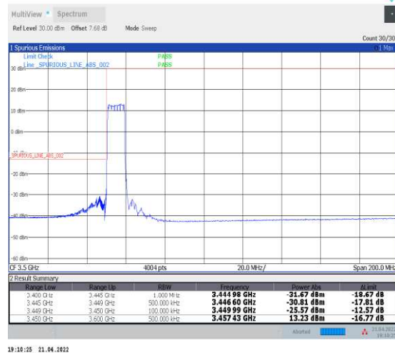
1-N78-3450-3550--30-10-L-3-DFT-PI2BPSK-Outer_Full-24@0-Ant1-PASS-see graph
