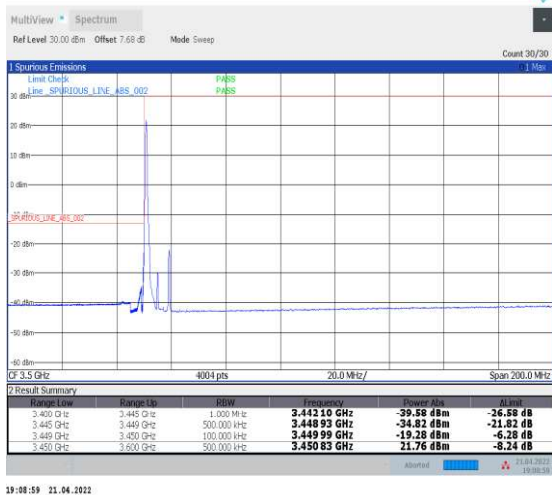
1-N78-3450-3550--30-10-L-1-DFT-PI2BPSK-Edge_1R_B_Left-1@0-Ant1-PASS-see graph
