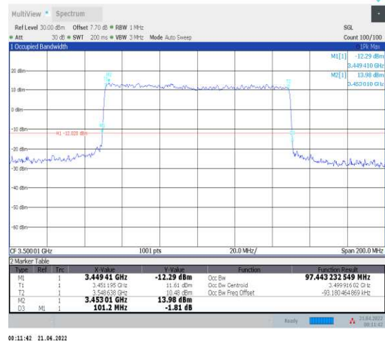
1-N78-3450-3550--30-100-L-6-CP-QPSK-Outer_F ull-273@0-Ant1-97.443-101.200-≤100-PASS
