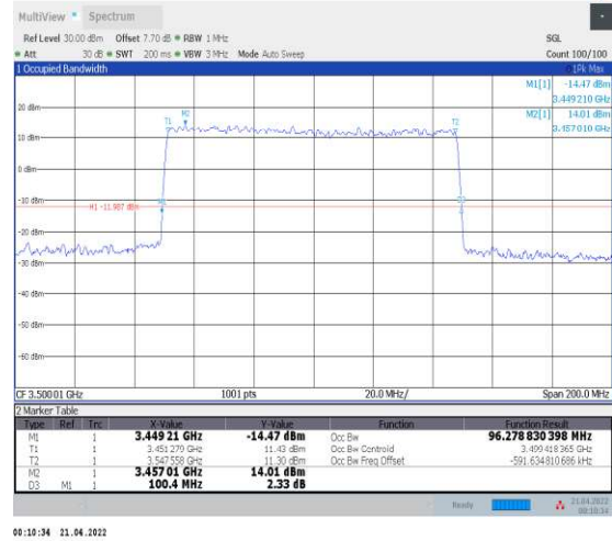
1-N78-3450-3550--30-100-L-4-DFT-64QAM-Outer_F ull-270@0-Ant1-96.279-100.400-≤100-PASS
