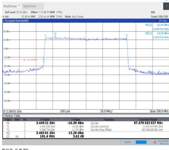
1-N78-3450-3550--30-100-L-7-CP-16QAM-Outer_Fu II-273@0-Ant1-97.58-101.400-≤100-PASS
