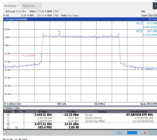
1-N78-3450-3550--30-100-L-8-CP-64QAM-Outer_Fu II-273@0-Ant1-97.481-101.400-≤100-PASS
