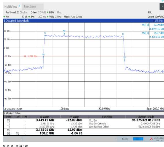
1-N78-3450-3550--30-100-M-1-DFT-QPSK-Outer_F ull-270@0-Ant1-96.375-100.200-≤100-PASS
