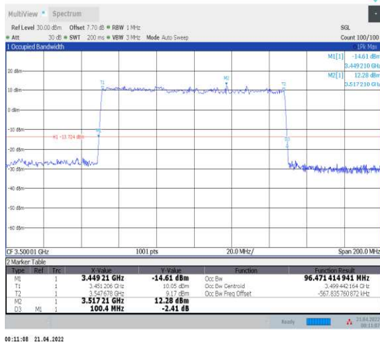
1-N78-3450-3550--30-100-L-5-DFT-256QAM-Outer_F ull-270@0-Ant1-96.471-100.400-≤100-PASS
