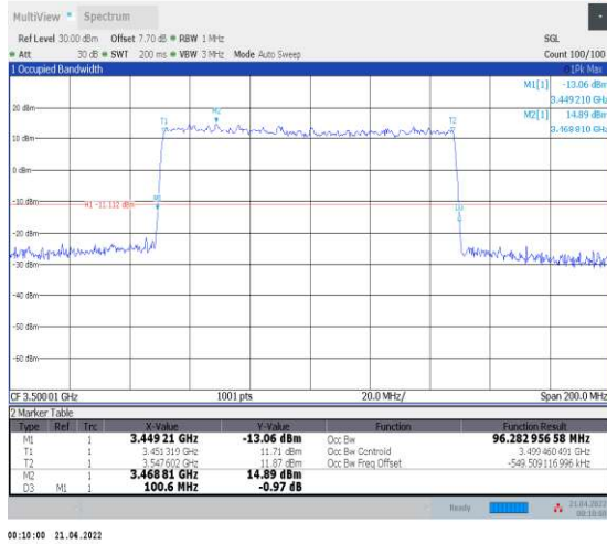
1-N78-3450-3550--30-100-L-3-DFT-16QAM-Outer_F ull-270@0-Ant1-96.283-100.600-≤100-PASS
