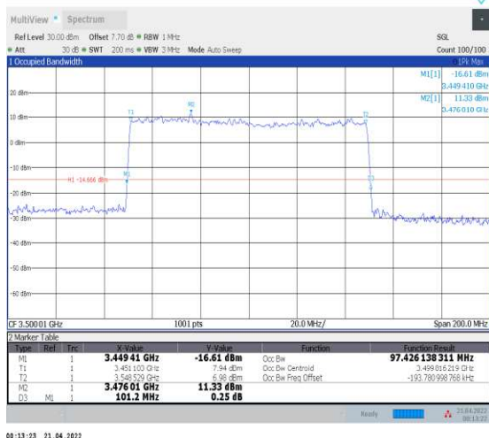
1-N78-3450-3550--30-100-L-9-CP-256QAM-Outer_F ull-273@0-Ant1-97.426-101.200-≤100-PASS
