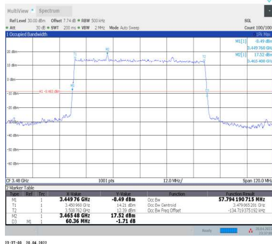
1-N78-3450-3550--30-60-L-2-DFT-PI2BPSK-Outer_ Full-162@0-Ant1-57.794-60.360-≤60-PASS
