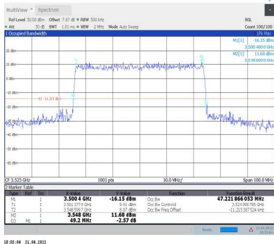
1-N78-3450-3550--30-50-H-8-CP-64QAM-Outer_Full -133@0-Ant1-47.222-49.200-≤50-PASS
