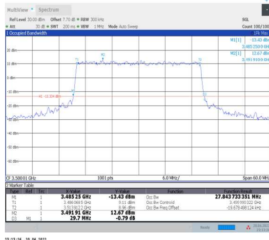
1-N78-3450-3550--30-30-M-8-CP-64QAM-Outer_Full I-78@0-Ant1-27.844-29.700≤30-PASS
