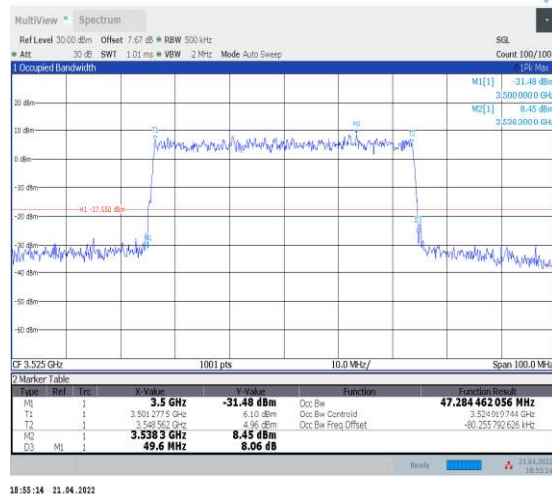
1-N78-3450-3550--30-50-H-9-CP-256QAM-Outer_F ull-133@0-Ant1-47.284-49.600-≤50-PASS
