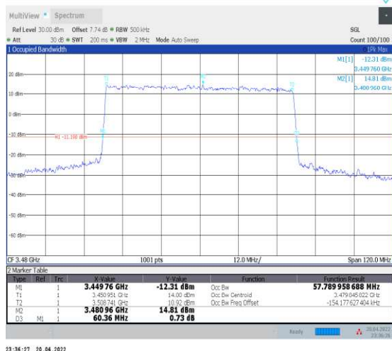
1-N78-3450-3550--30-60-L-1-DFT-QPSK-Outer_Full- 162@0-Ant1-57.79-60.360-≤60-PASS
