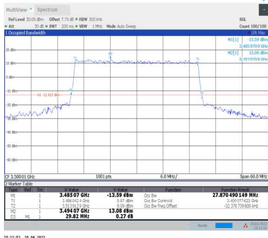
1-N78-3450-3550--30-30-M-7-CP-16QAM-Outer_Full -78@0-Ant1-27.87-29.820-≤30-PASS
