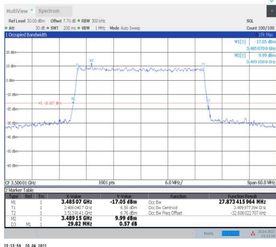
1-N78-3450-3550--30-30-M-9-CP-256QAM-Outer_F ull-78@0-Ant1-27.873-29.820-≤30-PASS
