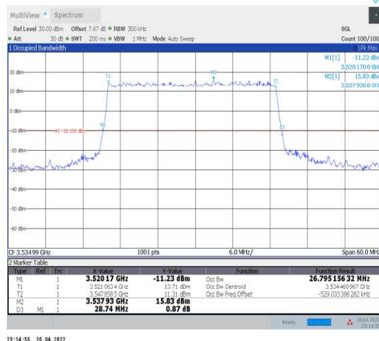
1-N78-3450-3550--30-30-H-1-DFT-QPSK-Outer_Full -75@0-Ant1-26.795-28.740-≤30-PASS
