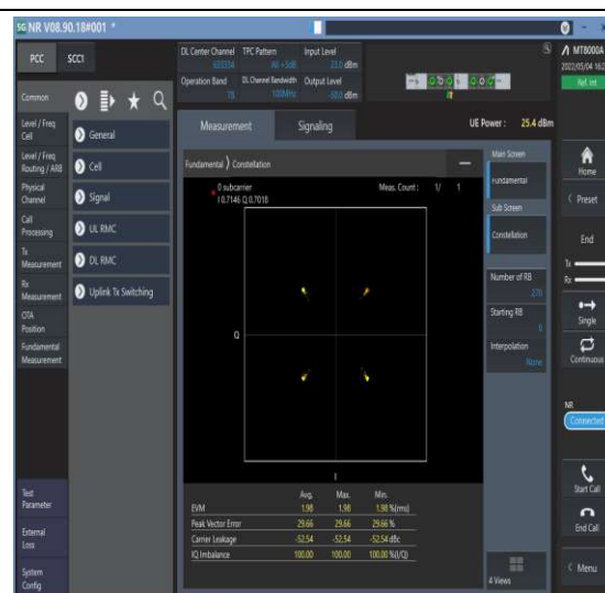
1-N78-3450-3550--30-100-M-2-DFT-QPSK-Outer_Full-270@0-Ant1-see graph-PASS
