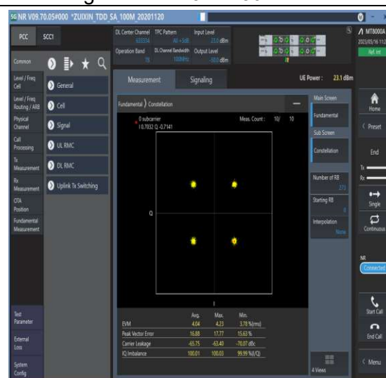
1-N78-3450-3550-PC1-30-100-M-6-CP-QPSK-Outer_Full-273@0-Ant1-see graph-PASS
