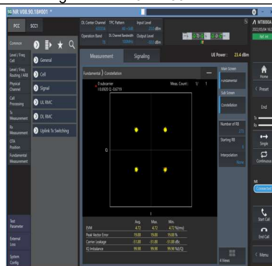
1-N78-3450-3550--30-100-M-6-CP-QPSK-Outer_Full-273@0-Ant1-see graph-PASS
