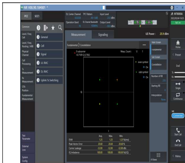
1-N78-3450-3550--30-100-M-1-DFT-PI2BPSK-Outer_Full-270@0-Ant1-see graph-PASS
