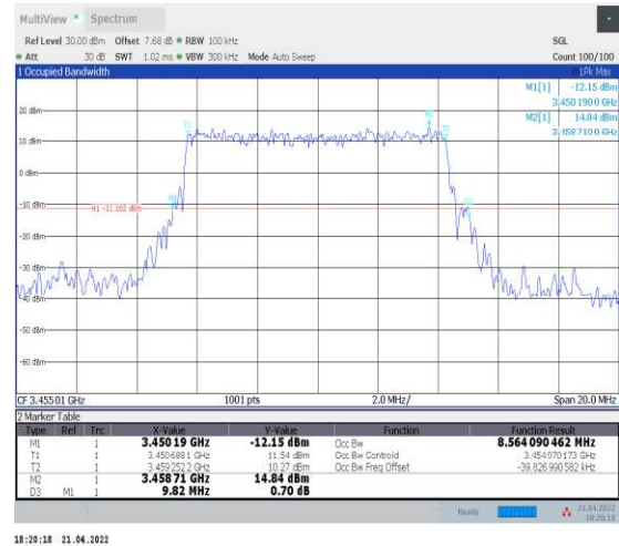
1-N78-3450-3550--30-10-L-2-DFT-PI2BPSK-Out_Full-24@0-Ant1-8.564-9.820-≤10-PASS
