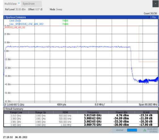
1-N77-3700-3980--30-70-H-3-DFT-PI2BPSK-Outer _Full-180@0-Ant1-PASS-see graph
