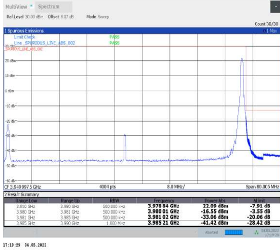
1-N77-3700-3980--30-70-H-2-DFT-PI2BPSK-Edge_1R B_Right-1@188-Ant1-PASS-see graph
