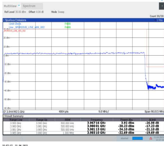
1-N77-3700-3980--30-80-H-3-DFT-PI2BPSK-Outer _Full-216@0-Ant1-PASS-see graph
