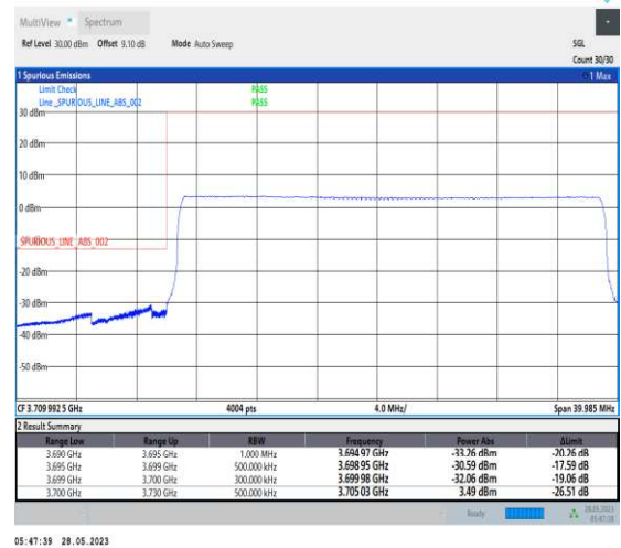
1-N77-3700-3980-PC1-30-30-L-6-CP-QPSK-Outer_Full-78@0-Ant1-1--PASS-see graph
