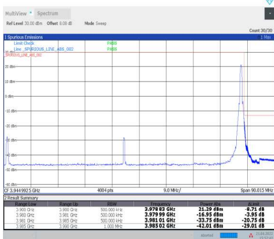
1-N77-3700-3980--30-80-H-5-CP-QPSK-Edge_1RB_R ight-1@216-Ant1-PASS-see graph
