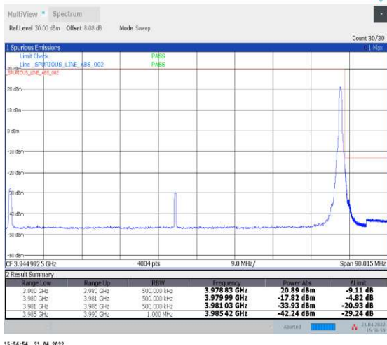
1-N77-3700-3980--30-80-H-2-DFT-PI2BPSK-Edge_1R B_Right-1@216-Ant1-PASS-see graph
