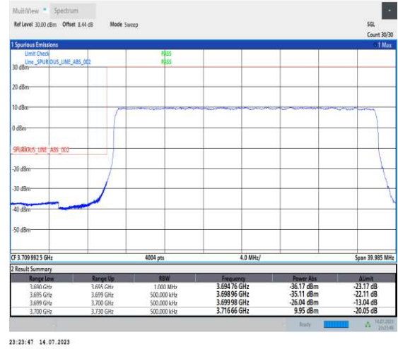
1-N77-3700-3980-PC1-30-30-L-3-DFT-PI2BPSK-Outer_Full-75@0-Ant1-1--PASS-see graph
