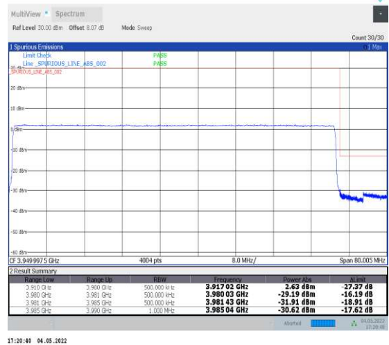
1-N77-3700-3980--30-70-H-6-CP-QPSK-Outer_Fu ll-189@0-Ant1-PASS-see graph
