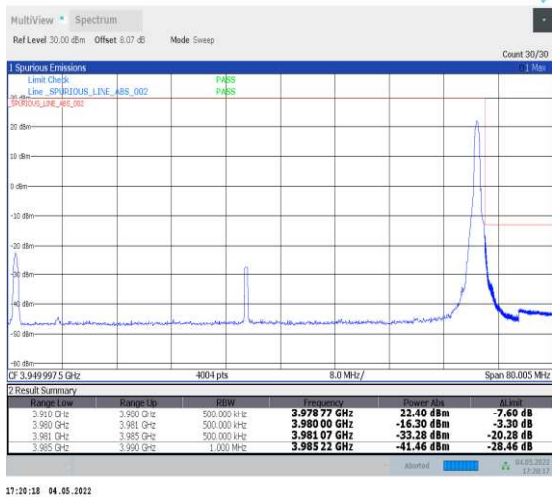
1-N77-3700-3980--30-70-H-5-CP-QPSK-Edge_1RB_R ight-1@188-Ant1-PASS-see graph
